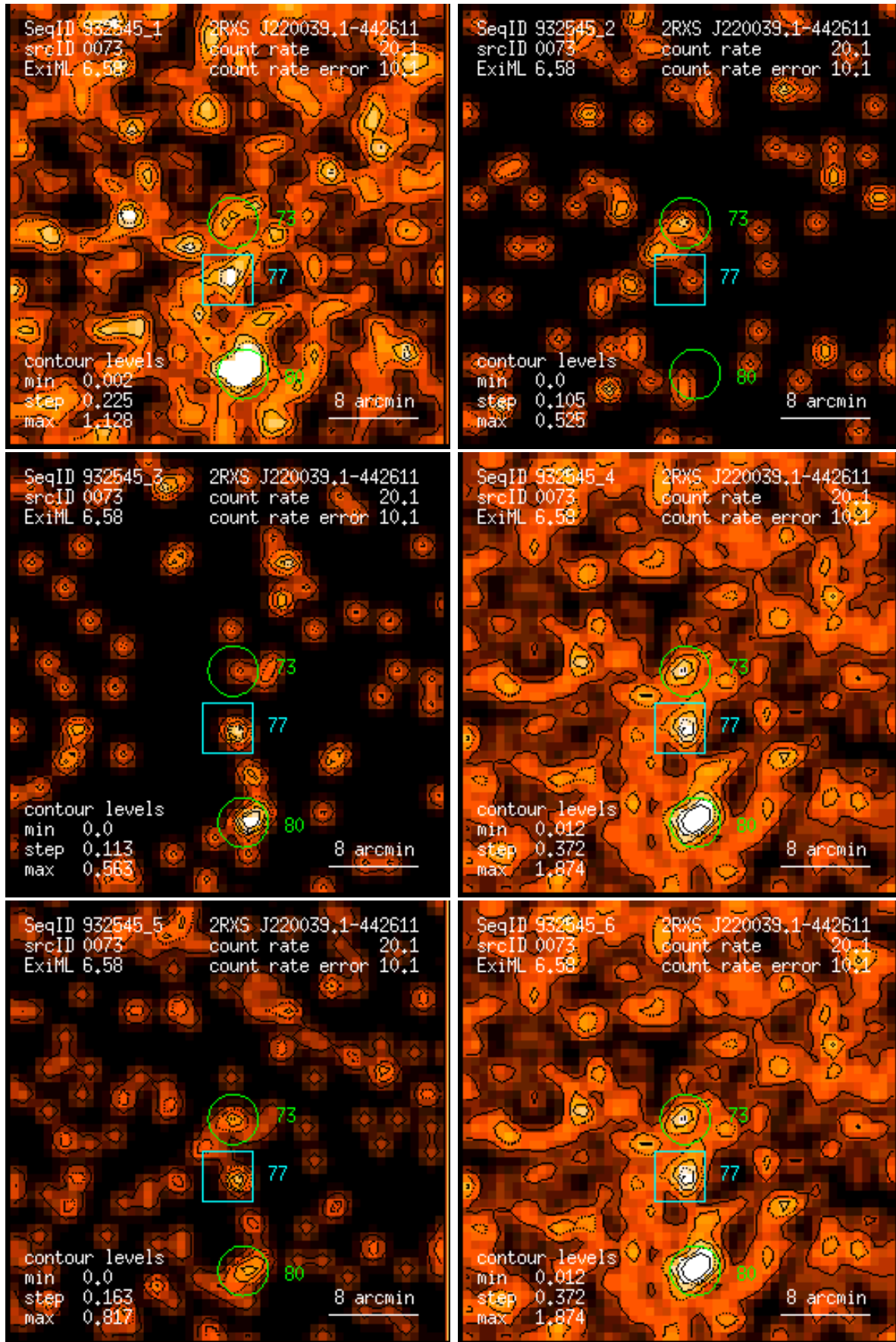
Figure 73: RASS 932545: detection 0073: band rate images, Gaussian filter: (1) PSPC channels 11 – 41, (2) 52 – 90, (3) 91 – 201, (4) 11 – 235, (5) 52 – 201, (6) 11 – 201. Broad band rates in counts/ks. Band rate contour levels in counts/ks/arcmin 2 .
