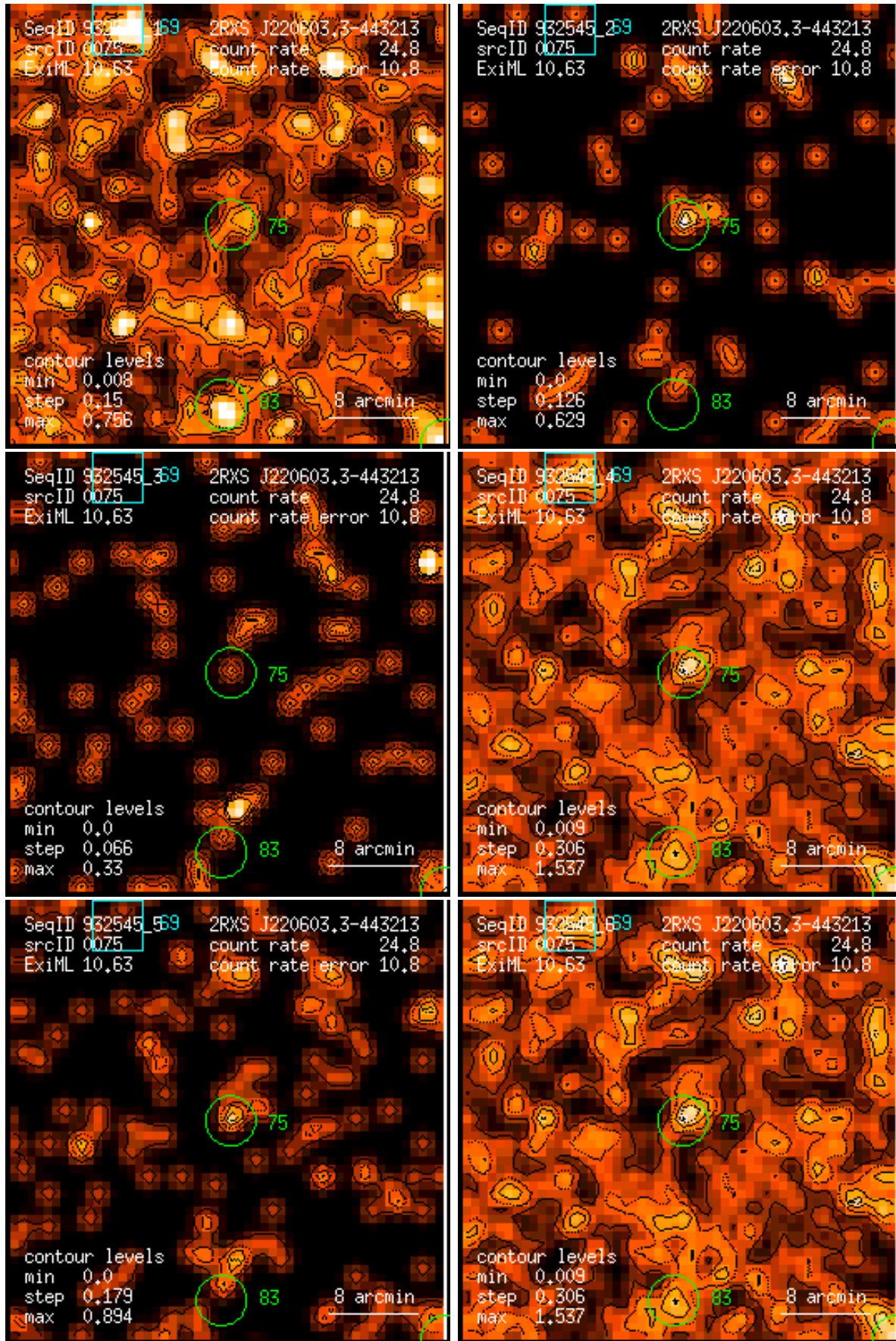
Figure 75: RASS 932545: detection 0075: band rate images, Gaussian filter: (1) PSPC channels 11 – 41, (2) 52 – 90, (3) 91 – 201, (4) 11 – 235, (5) 52 – 201, (6) 11 – 201. Broad band rates in counts/ks. Band rate contour levels in counts/ks/arcmin 2 .
