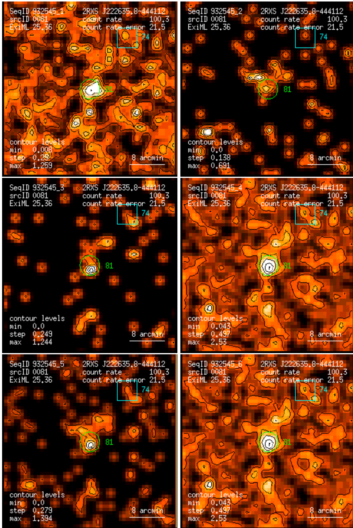
Figure 81: RASS 932545: detection 0081: band rate images, Gaussian filter: (1) PSPC channels 11 – 41, (2) 52 – 90, (3) 91 – 201, (4) 11 – 235, (5) 52 – 201, (6) 11 – 201. Broad band rates in counts/ks. Band rate contour levels in counts/ks/arcmin 2 .
