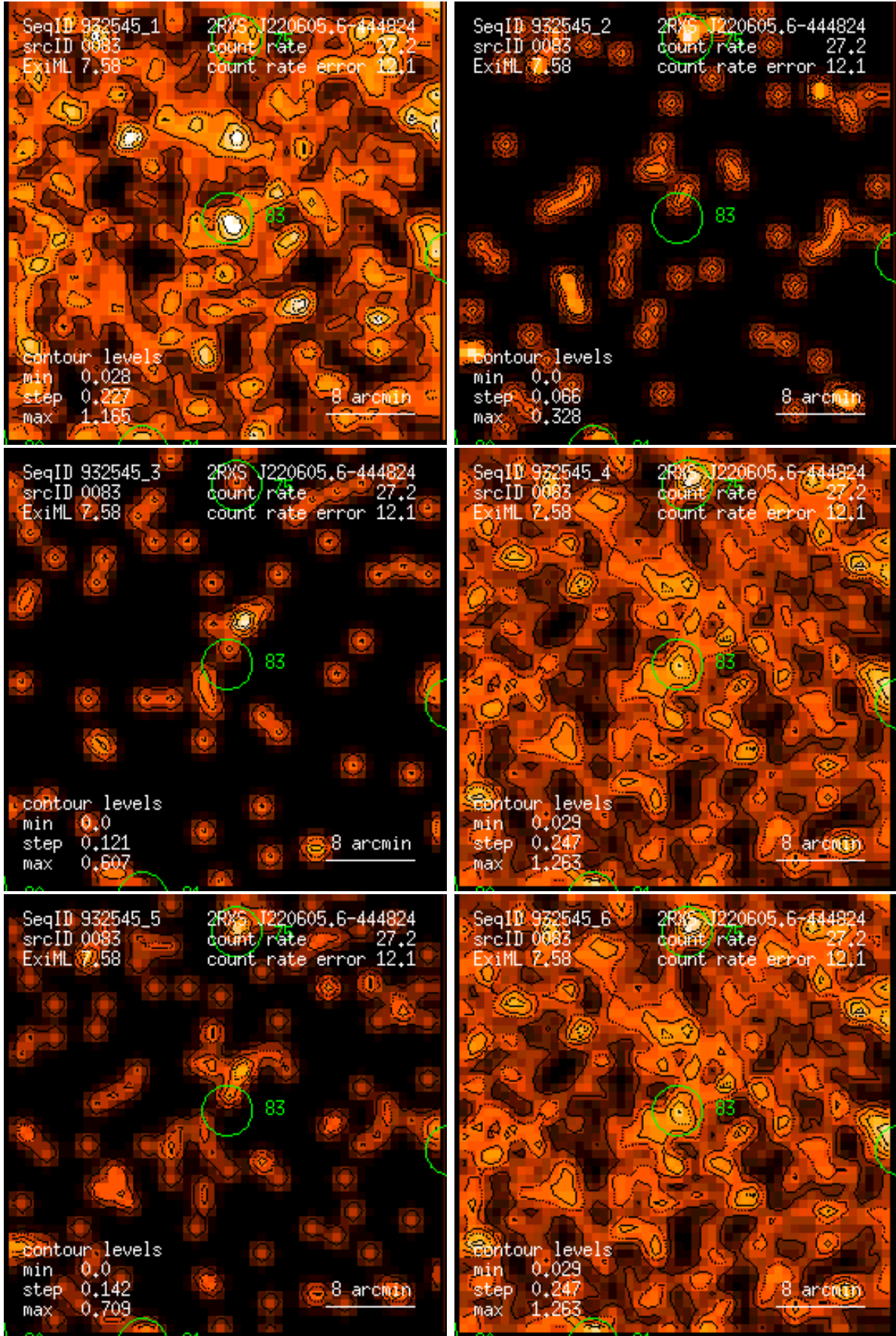
Figure 83: RASS 932545: detection 0083: band rate images, Gaussian filter: (1) PSPC channels 11 – 41, (2) 52 – 90, (3) 91 – 201, (4) 11 – 235, (5) 52 – 201, (6) 11 – 201. Broad band rates in counts/ks. Band rate contour levels in counts/ks/arcmin 2 .
