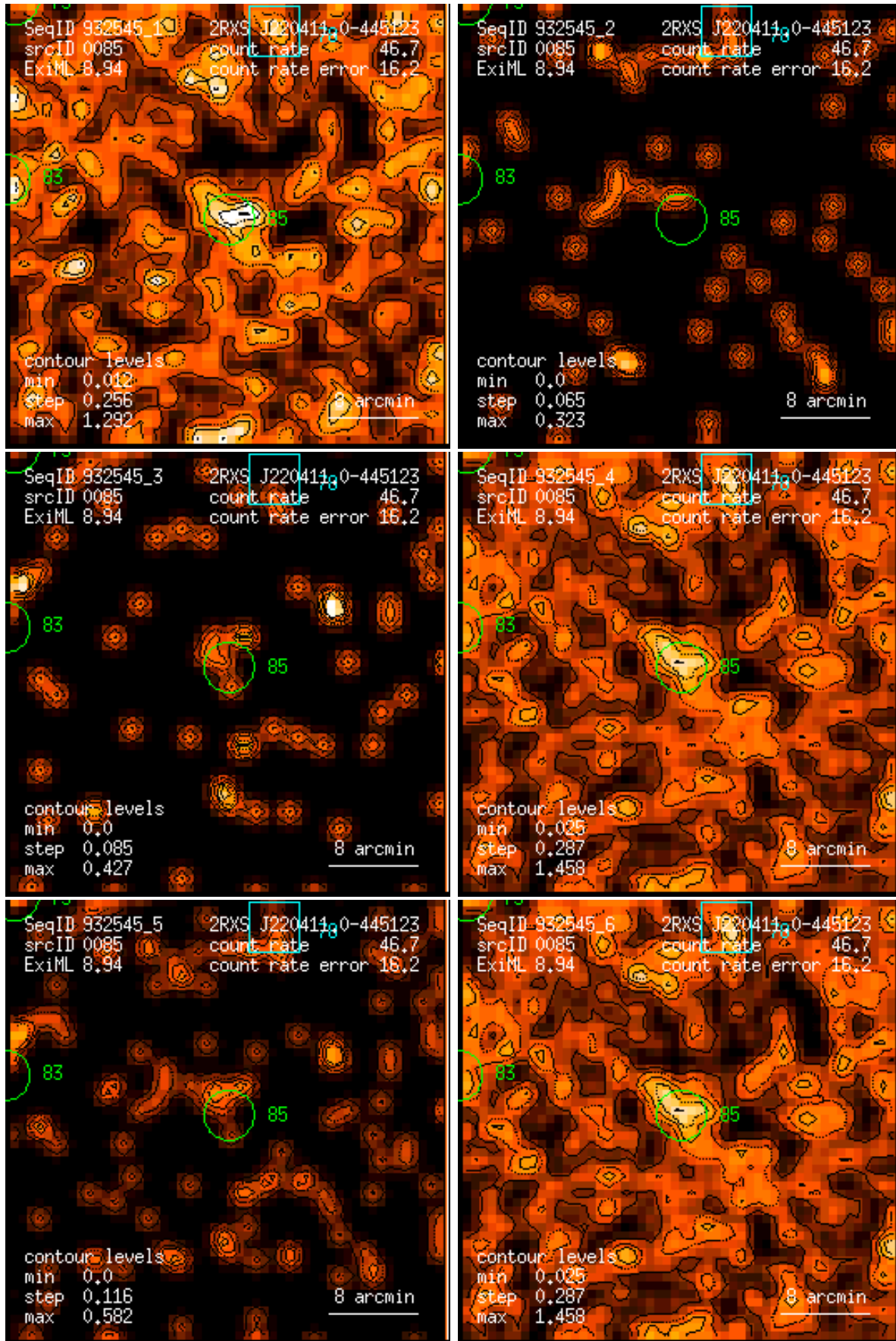
Figure 85: RASS 932545: detection 0085: band rate images, Gaussian filter: (1) PSPC channels 11 – 41, (2) 52 – 90, (3) 91 – 201, (4) 11 – 235, (5) 52 – 201, (6) 11 – 201. Broad band rates in counts/ks. Band rate contour levels in counts/ks/arcmin 2 .
