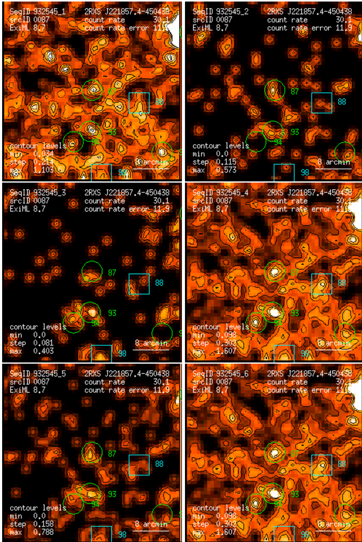
Figure 87: RASS 932545: detection 0087: band rate images, Gaussian filter: (1) PSPC channels 11 – 41, (2) 52 – 90, (3) 91 – 201, (4) 11 – 235, (5) 52 – 201, (6) 11 – 201. Broad band rates in counts/ks. Band rate contour levels in counts/ks/arcmin 2 .
