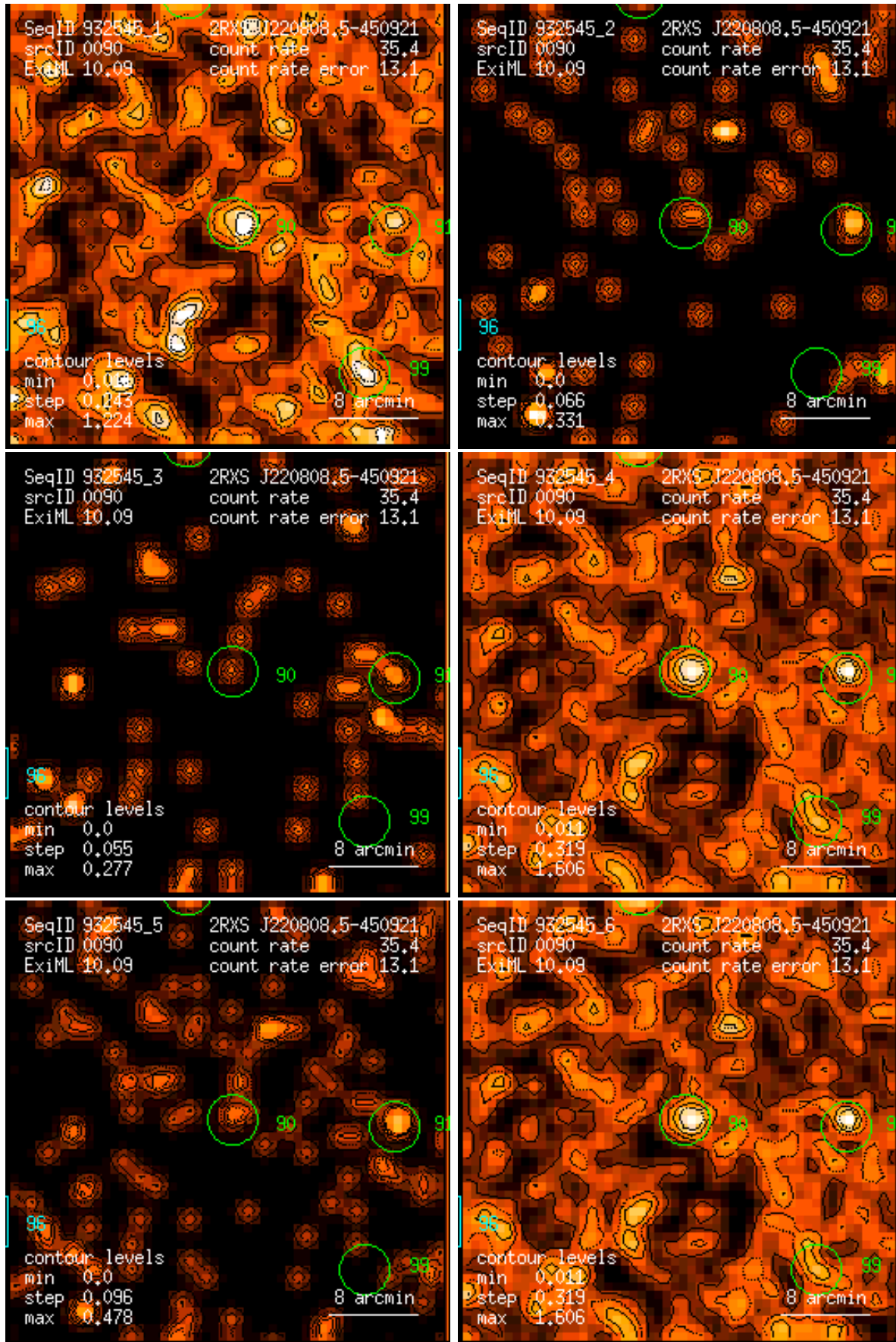
Figure 90: RASS 932545: detection 0090: band rate images, Gaussian filter: (1) PSPC channels 11 – 41, (2) 52 – 90, (3) 91 – 201, (4) 11 – 235, (5) 52 – 201, (6) 11 – 201. Broad band rates in counts/ks. Band rate contour levels in counts/ks/arcmin 2 .
