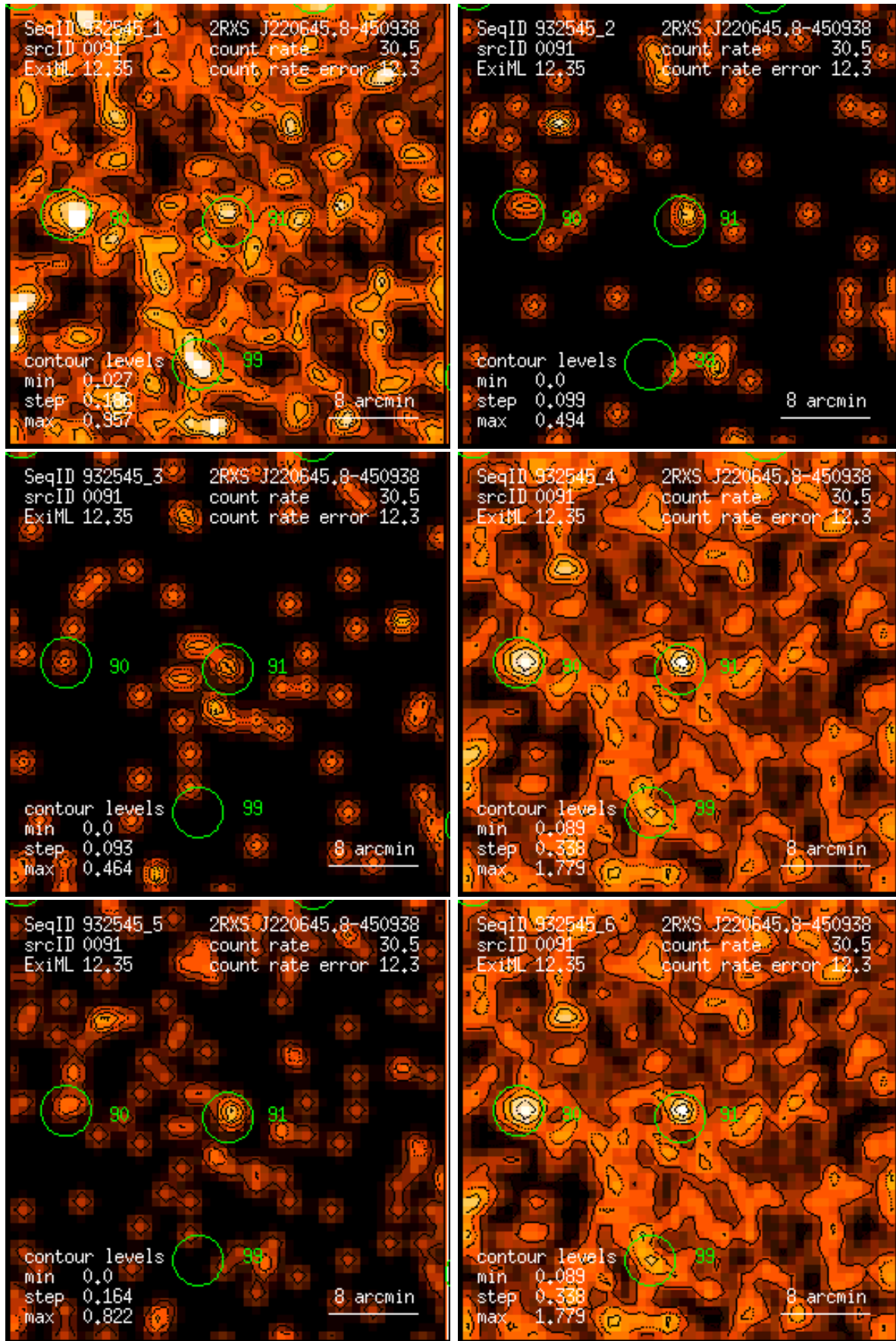
Figure 91: RASS 932545: detection 0091: band rate images, Gaussian filter: (1) PSPC channels 11 – 41, (2) 52 – 90, (3) 91 – 201, (4) 11 – 235, (5) 52 – 201, (6) 11 – 201. Broad band rates in counts/ks. Band rate contour levels in counts/ks/arcmin 2 .
