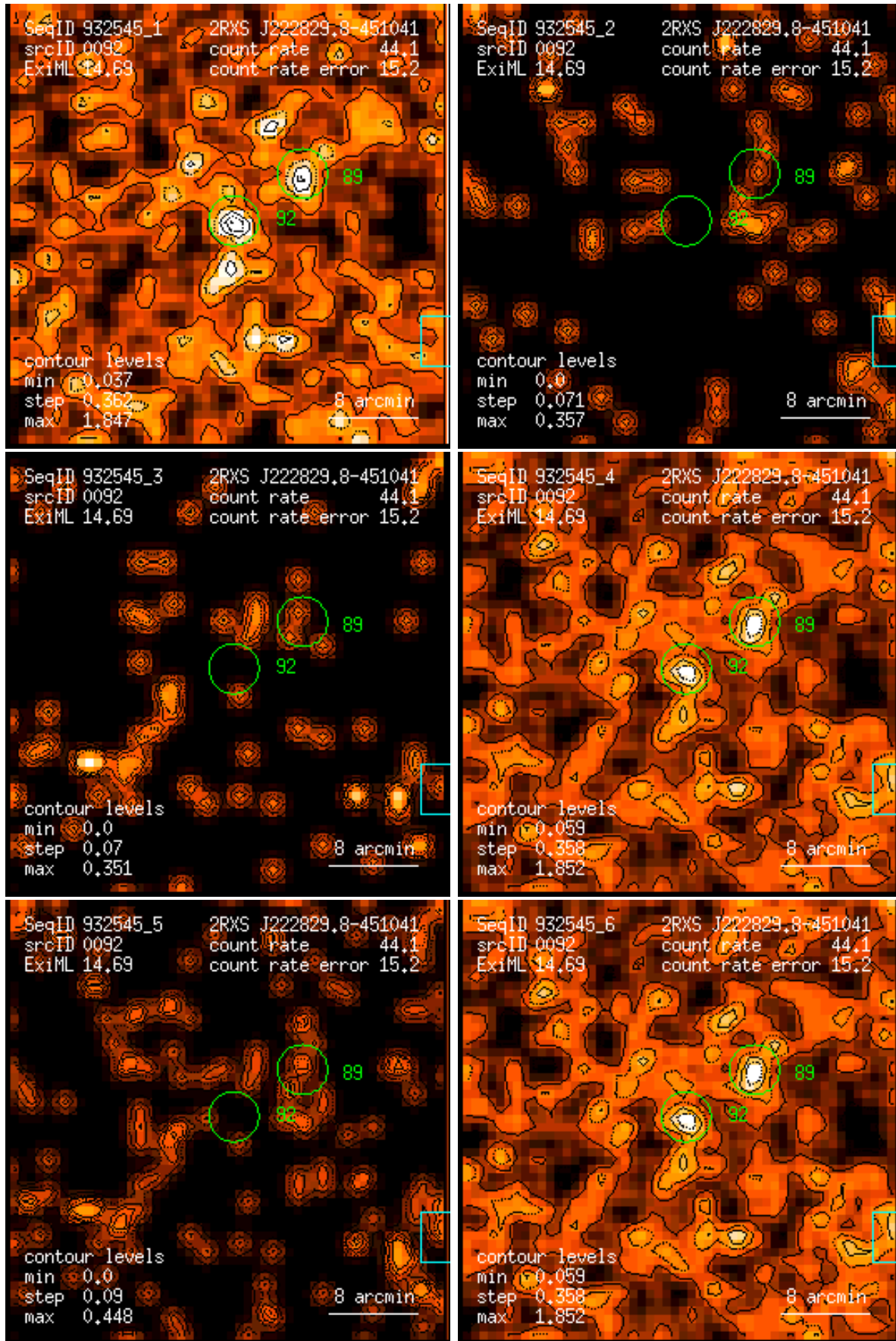
Figure 92: RASS 932545: detection 0092: band rate images, Gaussian filter: (1) PSPC channels 11 – 41, (2) 52 – 90, (3) 91 – 201, (4) 11 – 235, (5) 52 – 201, (6) 11 – 201. Broad band rates in counts/ks. Band rate contour levels in counts/ks/arcmin 2 .
