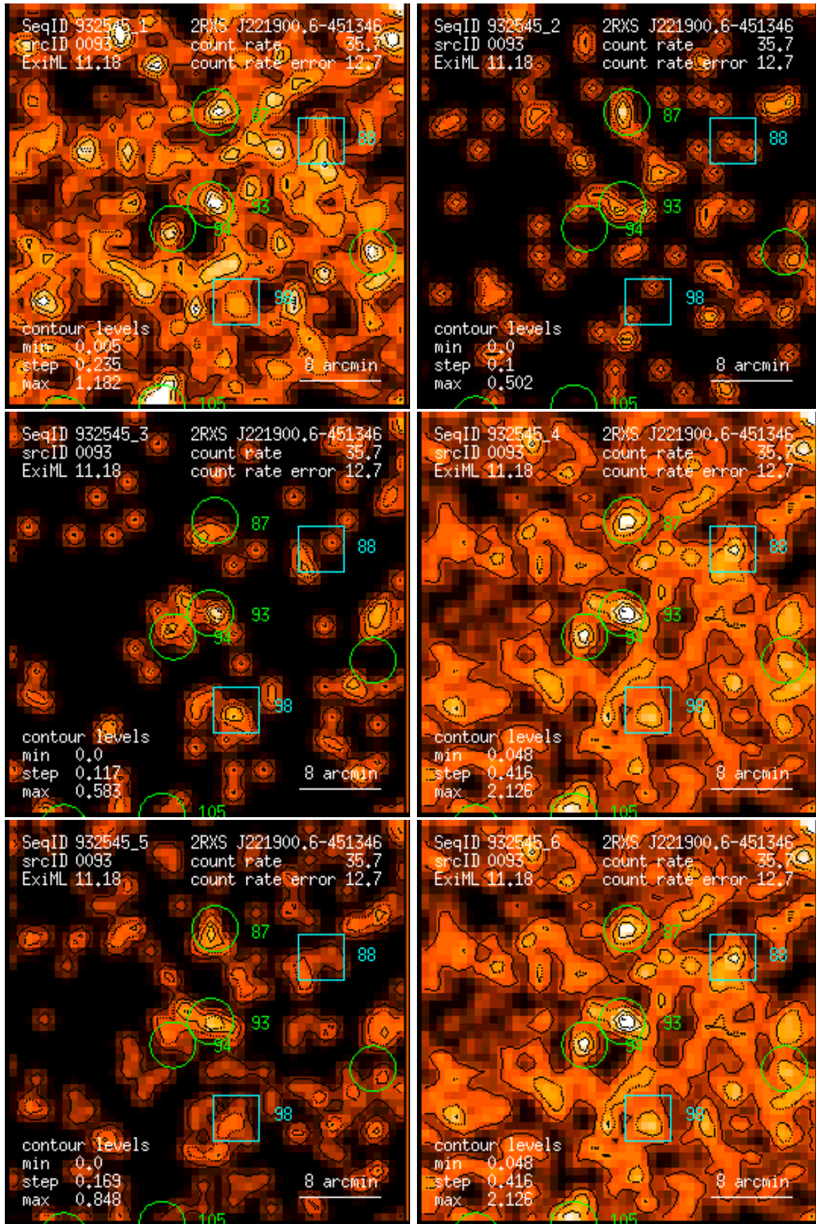
Figure 93: RASS 932545: detection 0093: band rate images, Gaussian filter: (1) PSPC channels 11 – 41, (2) 52 – 90, (3) 91 – 201, (4) 11 – 235, (5) 52 – 201, (6) 11 – 201. Broad band rates in counts/ks. Band rate contour levels in counts/ks/arcmin 2 .
