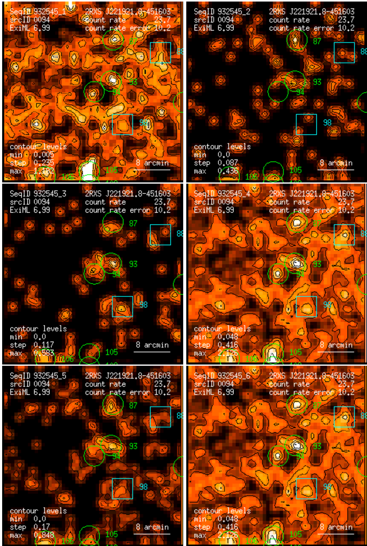
Figure 94: RASS 932545: detection 0094: band rate images, Gaussian filter: (1) PSPC channels 11 – 41, (2) 52 – 90, (3) 91 – 201, (4) 11 – 235, (5) 52 – 201, (6) 11 – 201. Broad band rates in counts/ks. Band rate contour levels in counts/ks/arcmin 2 .
