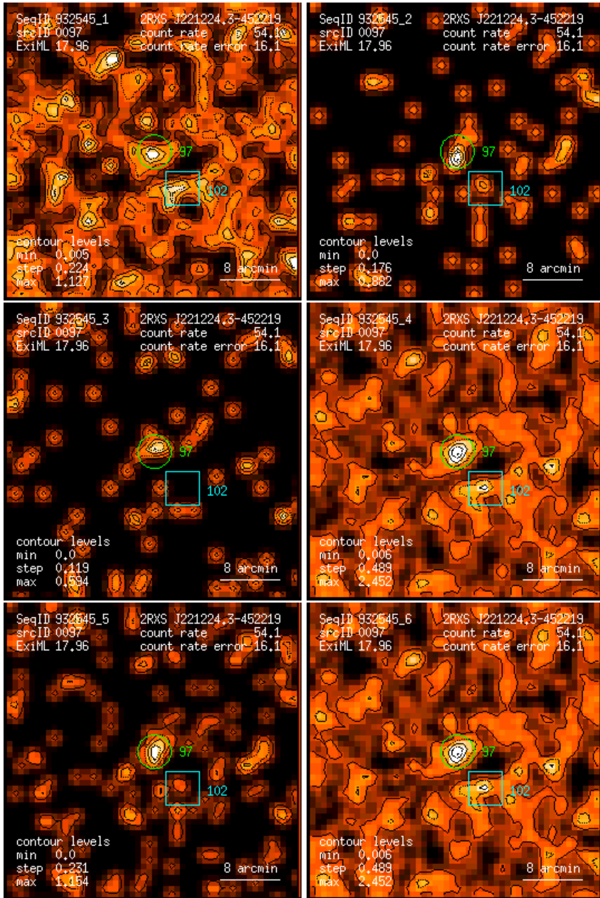
Figure 97: RASS 932545: detection 0097: band rate images, Gaussian filter: (1) PSPC channels 11 – 41, (2) 52 – 90, (3) 91 – 201, (4) 11 – 235, (5) 52 – 201, (6) 11 – 201. Broad band rates in counts/ks. Band rate contour levels in counts/ks/arcmin 2 .
