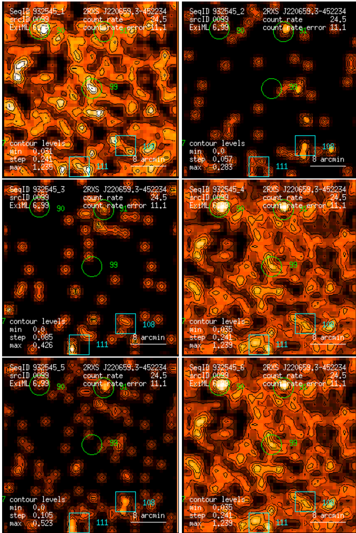
Figure 99: RASS 932545: detection 0099: band rate images, Gaussian filter: (1) PSPC channels 11 – 41, (2) 52 – 90, (3) 91 – 201, (4) 11 – 235, (5) 52 – 201, (6) 11 – 201. Broad band rates in counts/ks. Band rate contour levels in counts/ks/arcmin 2 .
