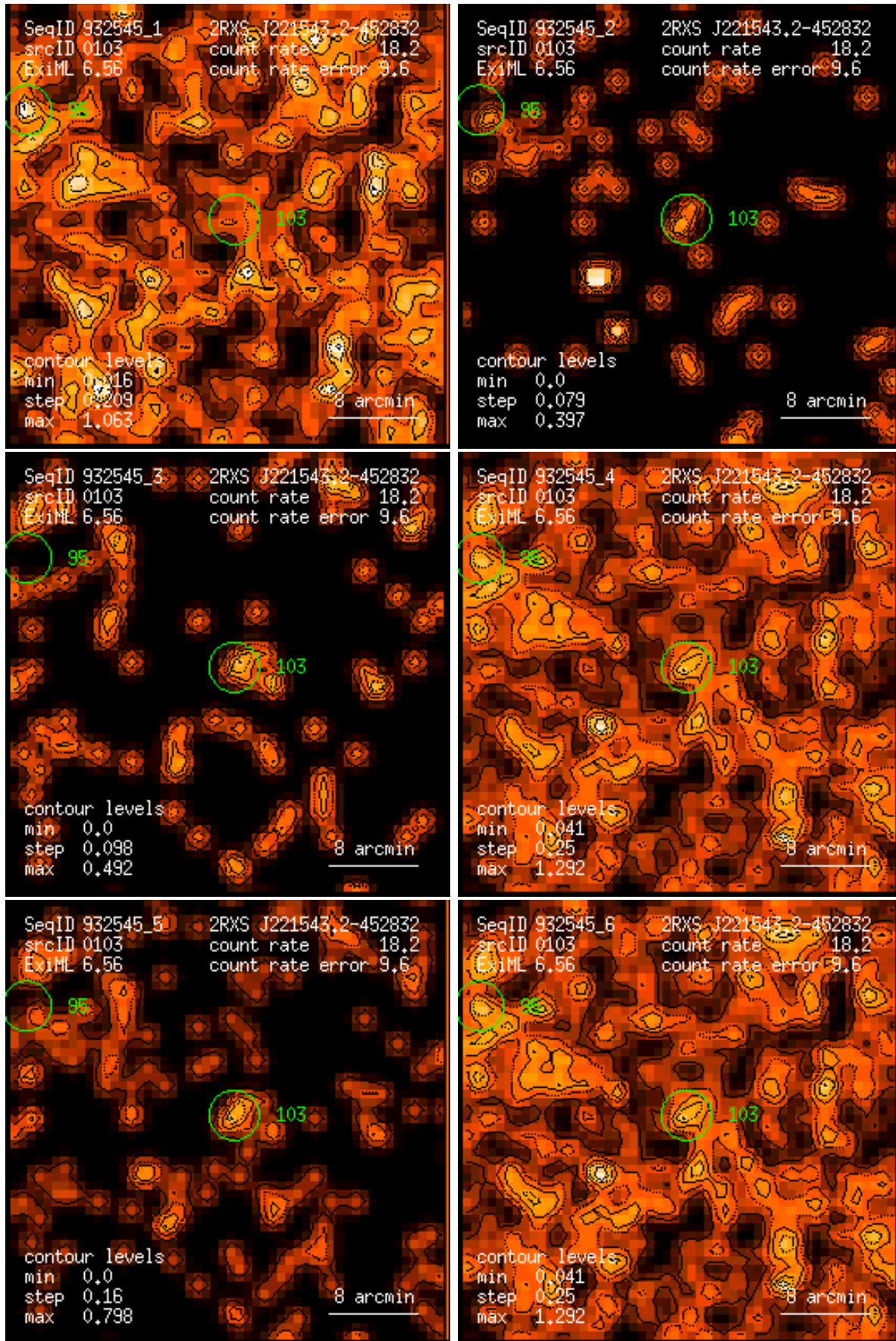
Figure 103: RASS 932545: detection 0103: band rate images, Gaussian filter: (1) PSPC channels 11 – 41, (2) 52 – 90, (3) 91 – 201, (4) 11 – 235, (5) 52 – 201, (6) 11 – 201. Broad band rates in counts/ks. Band rate contour levels in counts/ks/arcmin 2 .
