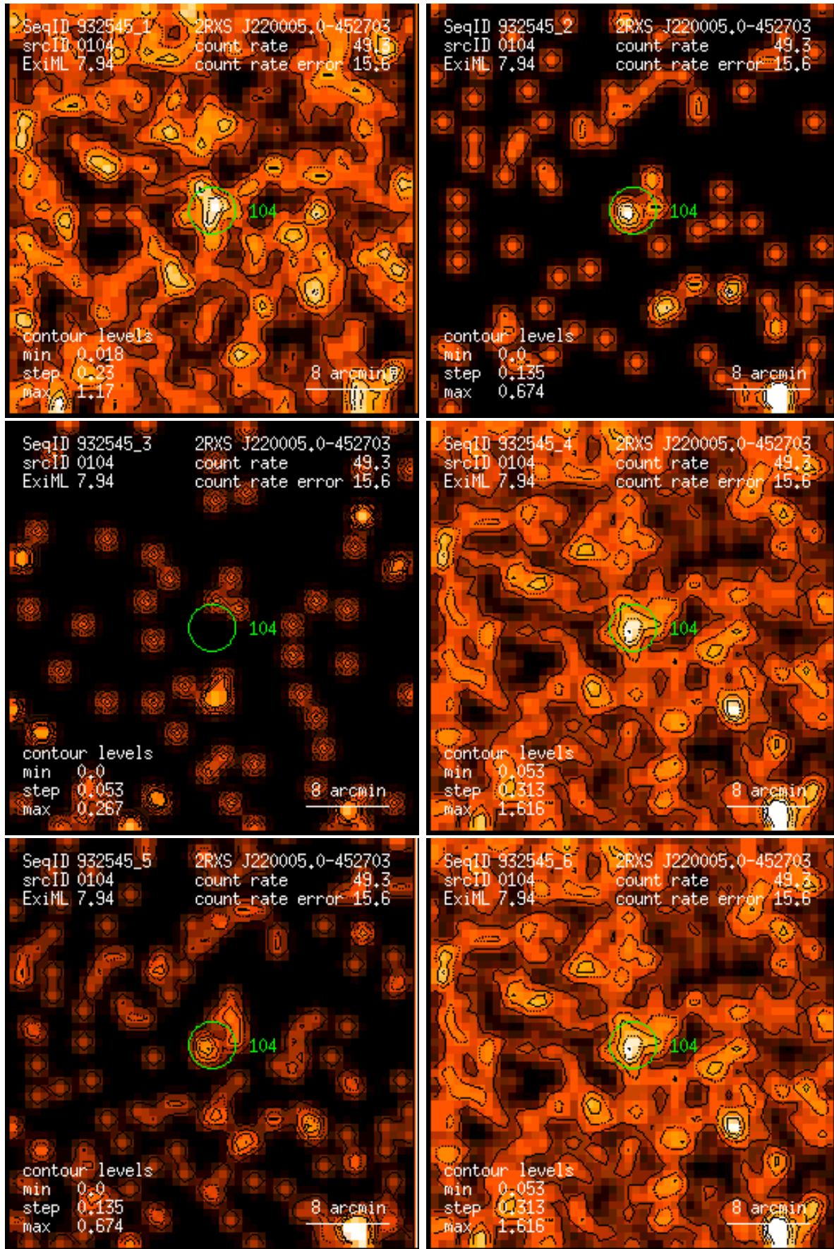
Figure 104: RASS 932545: detection 0104: band rate images, Gaussian filter: (1) PSPC channels 11 – 41, (2) 52 – 90, (3) 91 – 201, (4) 11 – 235, (5) 52 – 201, (6) 11 – 201. Broad band rates in counts/ks. Band rate contour levels in counts/ks/arcmin 2 .
