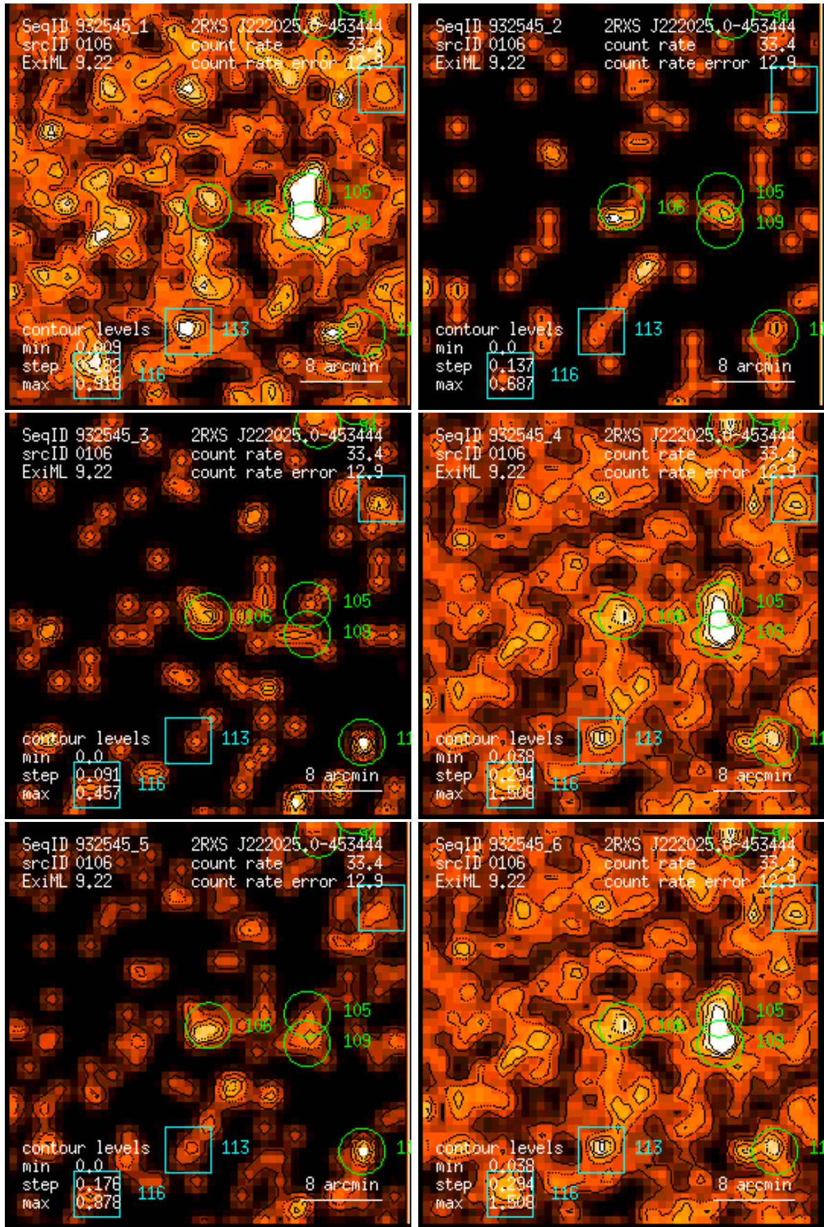
Figure 106: RASS 932545: detection 0106: band rate images, Gaussian filter: (1) PSPC channels 11 – 41, (2) 52 – 90, (3) 91 – 201, (4) 11 – 235, (5) 52 – 201, (6) 11 – 201. Broad band rates in counts/ks. Band rate contour levels in counts/ks/arcmin 2 .
