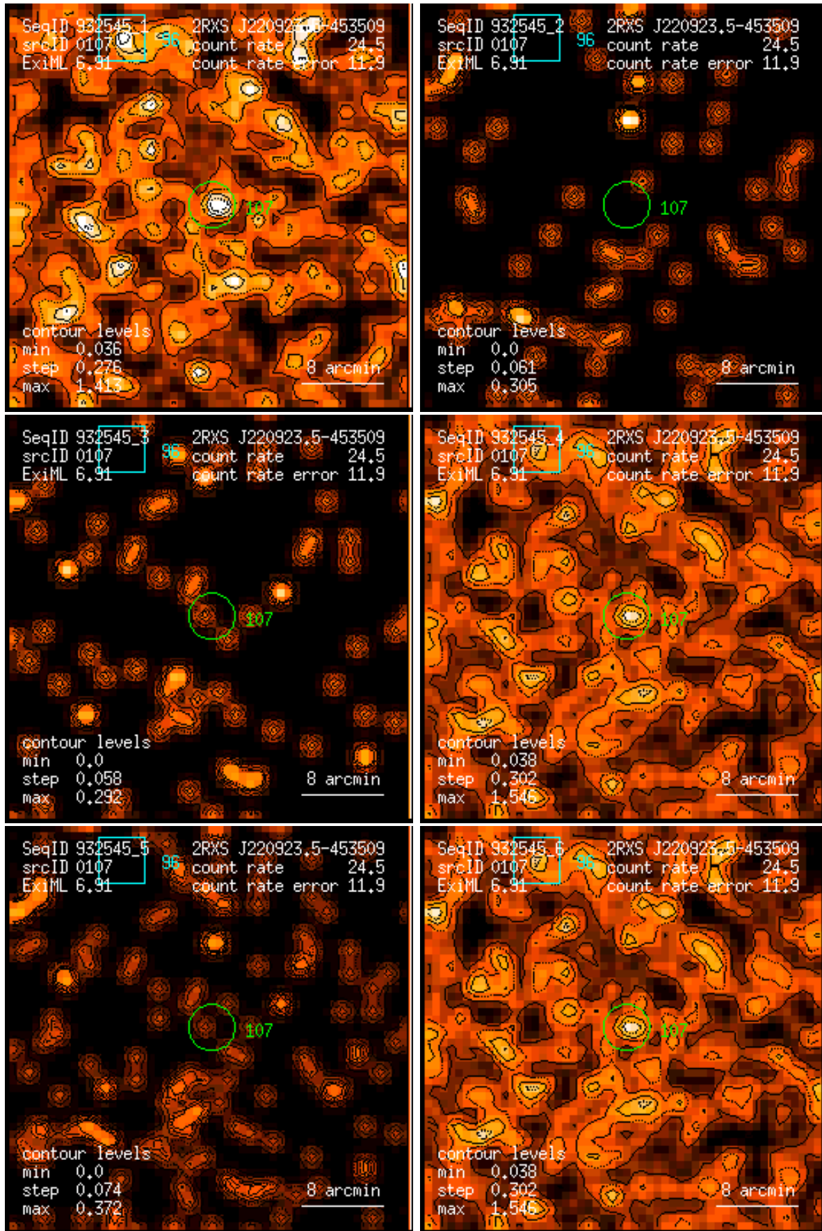
Figure 107: RASS 932545: detection 0107: band rate images, Gaussian filter: (1) PSPC channels 11 – 41, (2) 52 – 90, (3) 91 – 201, (4) 11 – 235, (5) 52 – 201, (6) 11 – 201. Broad band rates in counts/ks. Band rate contour levels in counts/ks/arcmin 2 .
