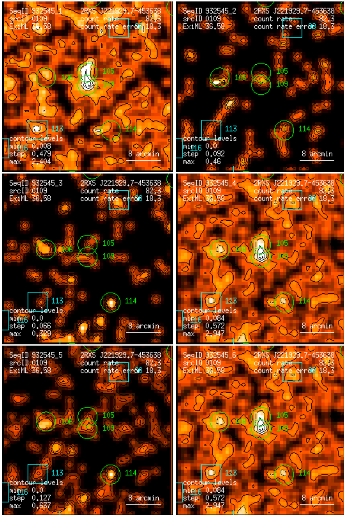
Figure 109: RASS 932545: detection 0109: band rate images, Gaussian filter: (1) PSPC channels 11 – 41, (2) 52 – 90, (3) 91 – 201, (4) 11 – 235, (5) 52 – 201, (6) 11 – 201. Broad band rates in counts/ks. Band rate contour levels in counts/ks/arcmin 2 .
