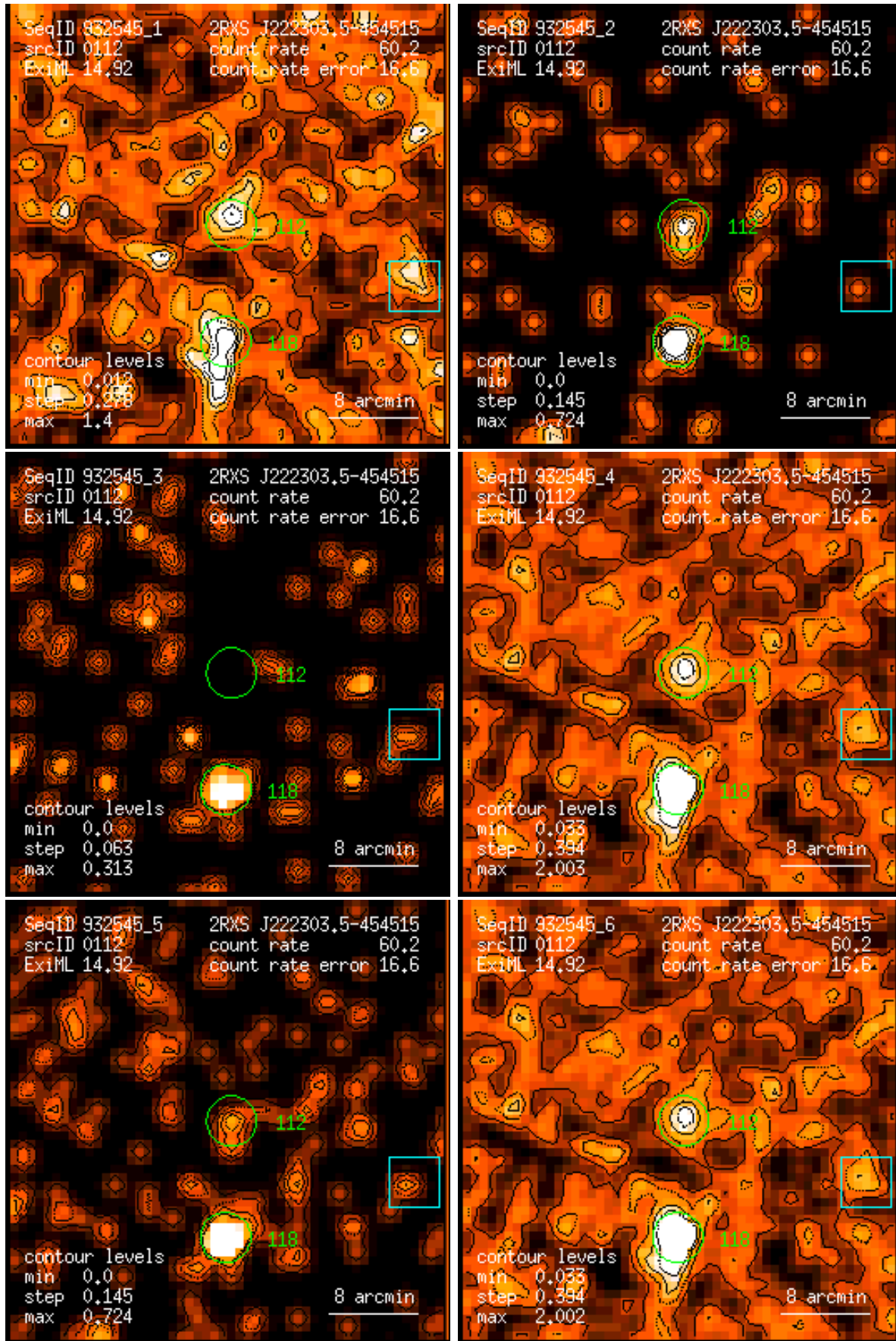
Figure 112: RASS 932545: detection 0112: band rate images, Gaussian filter: (1) PSPC channels 11 – 41, (2) 52 – 90, (3) 91 – 201, (4) 11 – 235, (5) 52 – 201, (6) 11 – 201. Broad band rates in counts/ks. Band rate contour levels in counts/ks/arcmin 2 .
