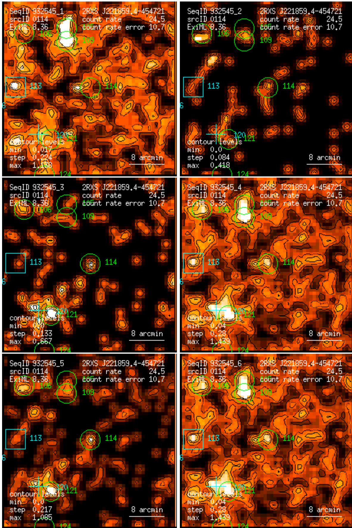
Figure 114: RASS 932545: detection 0114: band rate images, Gaussian filter: (1) PSPC channels 11 – 41, (2) 52 – 90, (3) 91 – 201, (4) 11 – 235, (5) 52 – 201, (6) 11 – 201. Broad band rates in counts/ks. Band rate contour levels in counts/ks/arcmin 2 .
