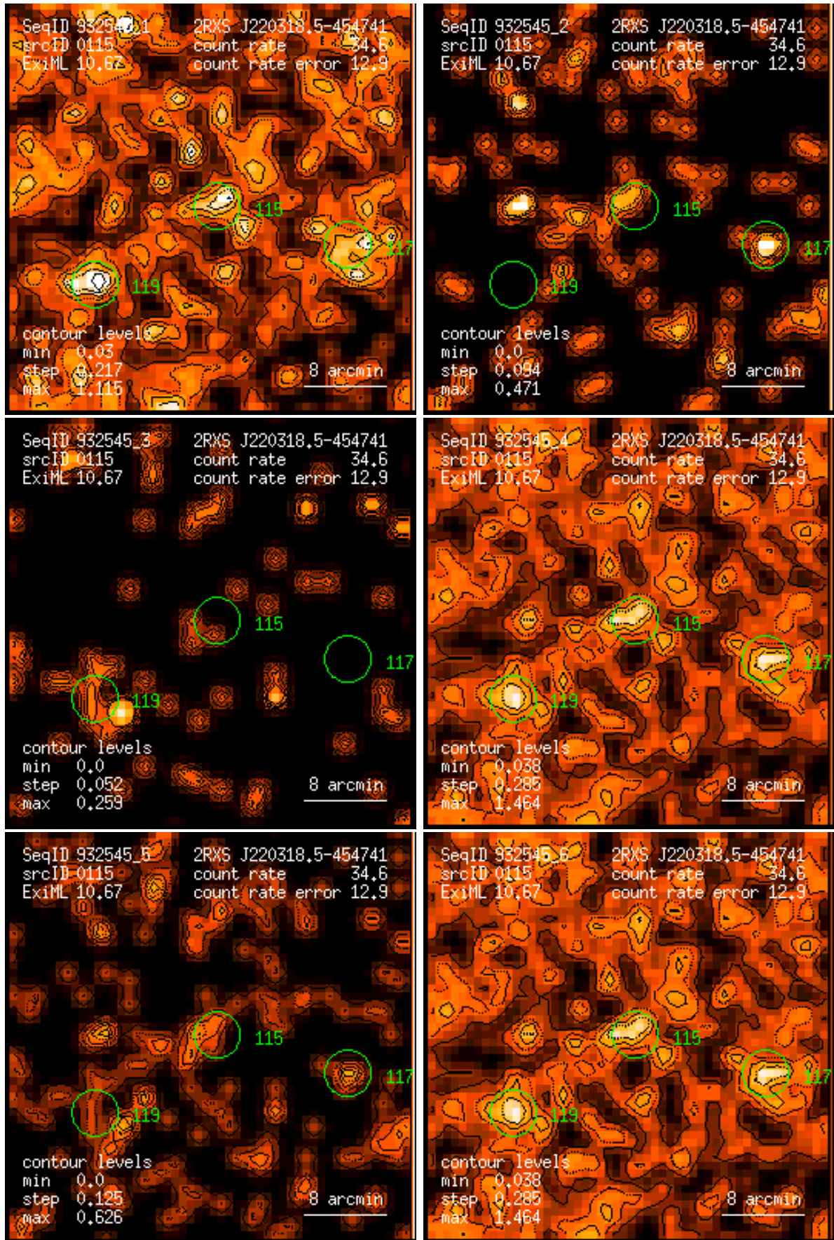
Figure 115: RASS 932545: detection 0115: band rate images, Gaussian filter: (1) PSPC channels 11 – 41, (2) 52 – 90, (3) 91 – 201, (4) 11 – 235, (5) 52 – 201, (6) 11 – 201. Broad band rates in counts/ks. Band rate contour levels in counts/ks/arcmin 2 .
