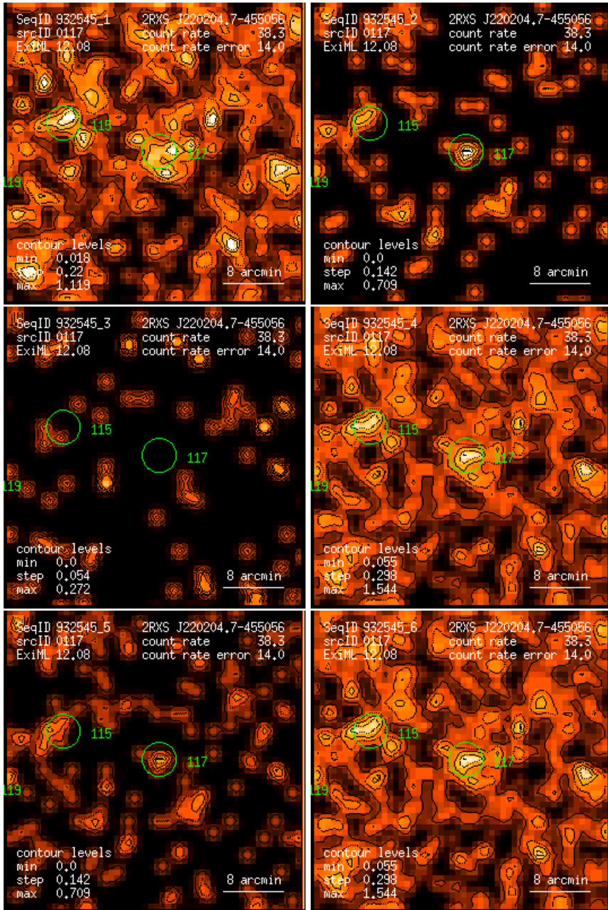
Figure 117: RASS 932545: detection 0117: band rate images, Gaussian filter: (1) PSPC channels 11 – 41, (2) 52 – 90, (3) 91 – 201, (4) 11 – 235, (5) 52 – 201, (6) 11 – 201. Broad band rates in counts/ks. Band rate contour levels in counts/ks/arcmin 2 .
