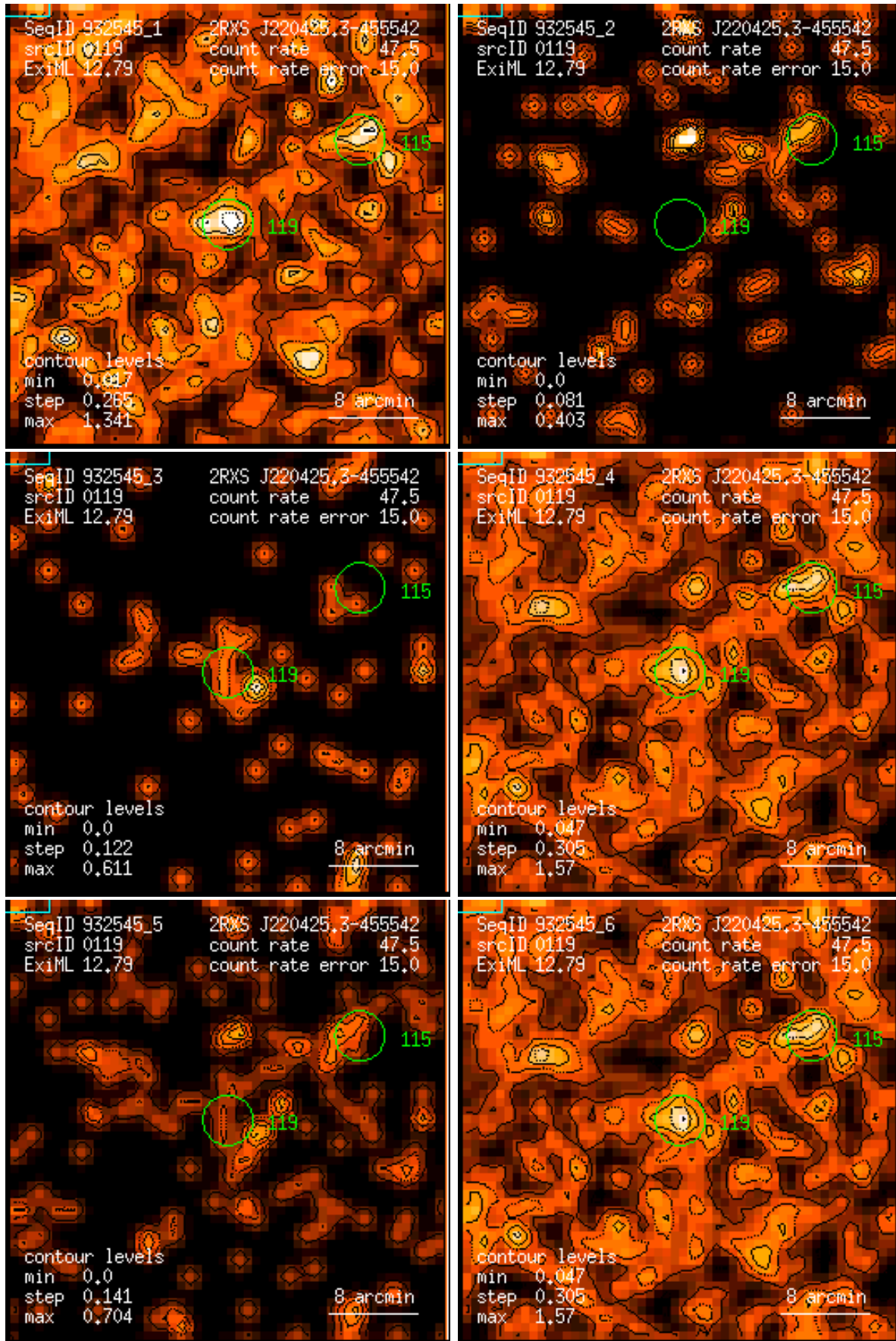
Figure 119: RASS 932545: detection 0119: band rate images, Gaussian filter: (1) PSPC channels 11 – 41, (2) 52 – 90, (3) 91 – 201, (4) 11 – 235, (5) 52 – 201, (6) 11 – 201. Broad band rates in counts/ks. Band rate contour levels in counts/ks/arcmin 2 .
