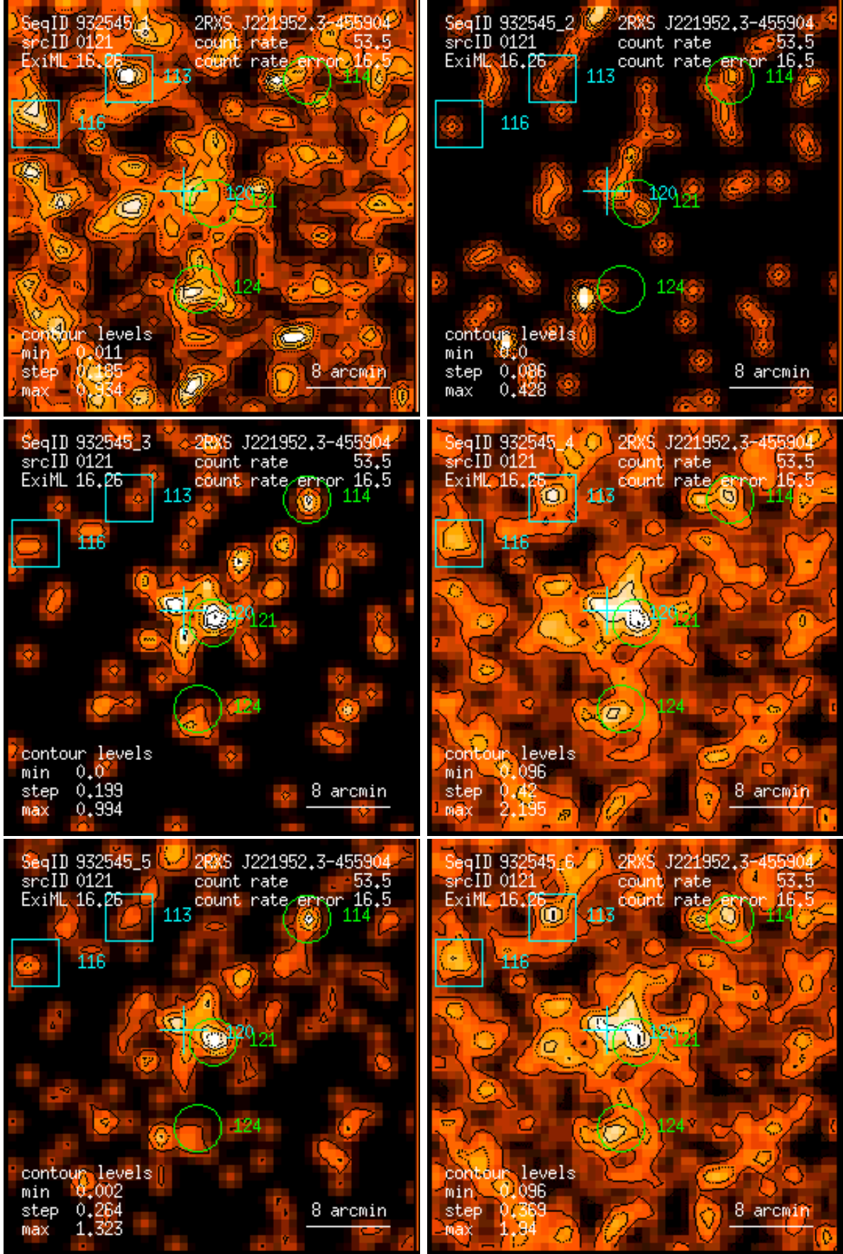
Figure 121: RASS 932545: detection 0121: band rate images, Gaussian filter: (1) PSPC channels 11 – 41, (2) 52 – 90, (3) 91 – 201, (4) 11 – 235, (5) 52 – 201, (6) 11 – 201. Broad band rates in counts/ks. Band rate contour levels in counts/ks/arcmin 2 .
