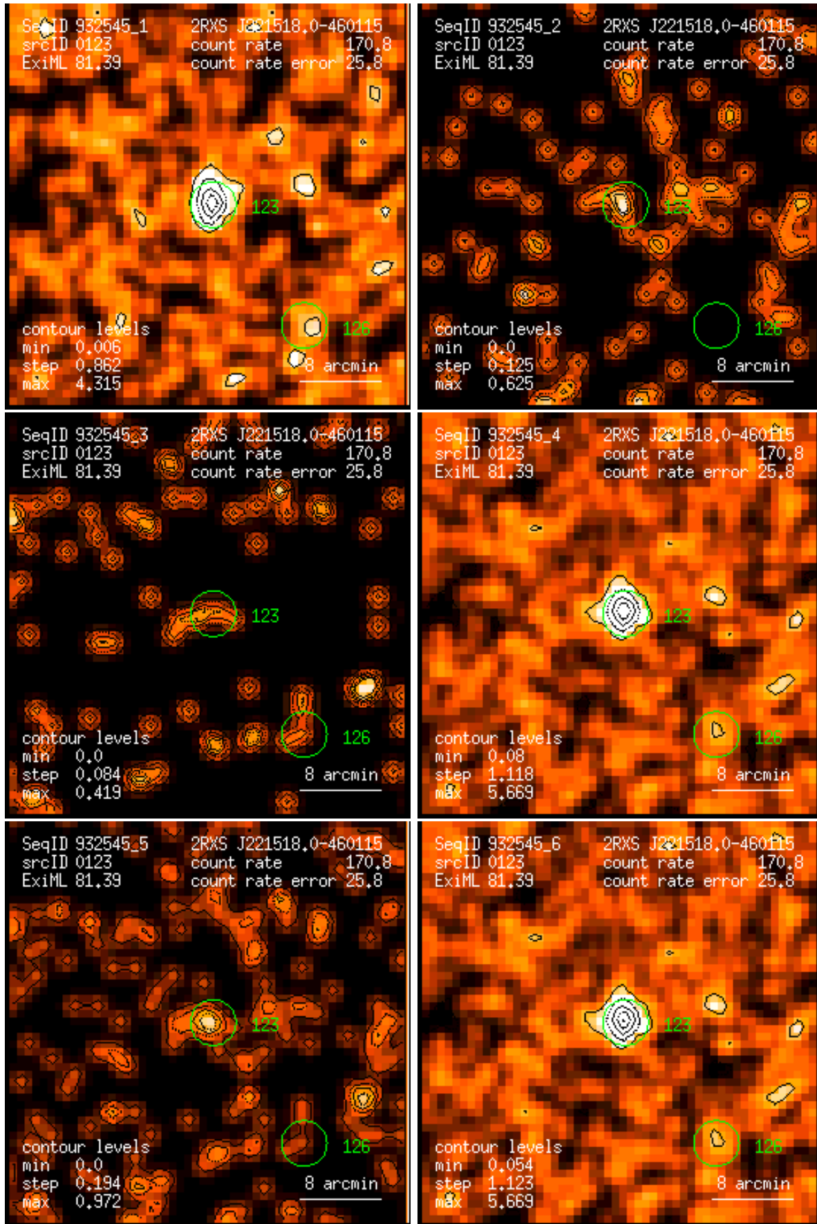
Figure 123: RASS 932545: detection 0123: band rate images, Gaussian filter: (1) PSPC channels 11 – 41, (2) 52 – 90, (3) 91 – 201, (4) 11 – 235, (5) 52 – 201, (6) 11 – 201. Broad band rates in counts/ks. Band rate contour levels in counts/ks/arcmin 2 .
