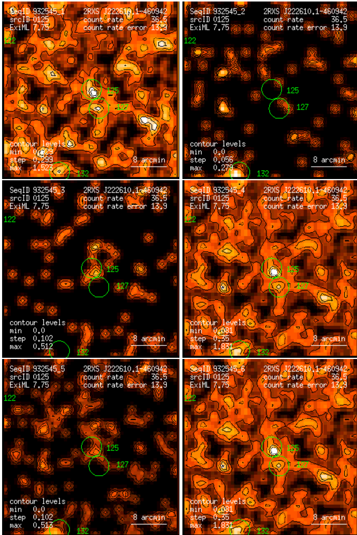
Figure 125: RASS 932545: detection 0125: band rate images, Gaussian filter: (1) PSPC channels 11 – 41, (2) 52 – 90, (3) 91 – 201, (4) 11 – 235, (5) 52 – 201, (6) 11 – 201. Broad band rates in counts/ks. Band rate contour levels in counts/ks/arcmin 2 .
