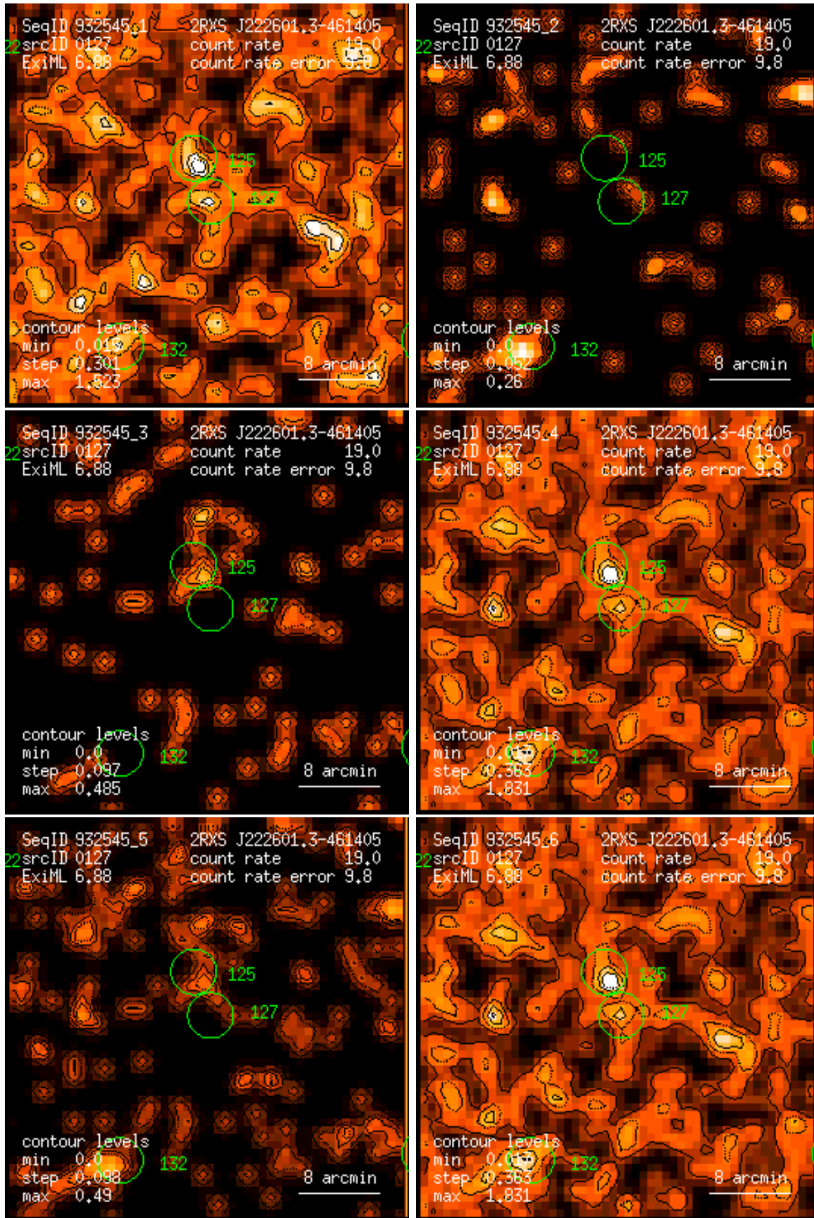
Figure 127: RASS 932545: detection 0127: band rate images, Gaussian filter: (1) PSPC channels 11 – 41, (2) 52 – 90, (3) 91 – 201, (4) 11 – 235, (5) 52 – 201, (6) 11 – 201. Broad band rates in counts/ks. Band rate contour levels in counts/ks/arcmin 2 .
