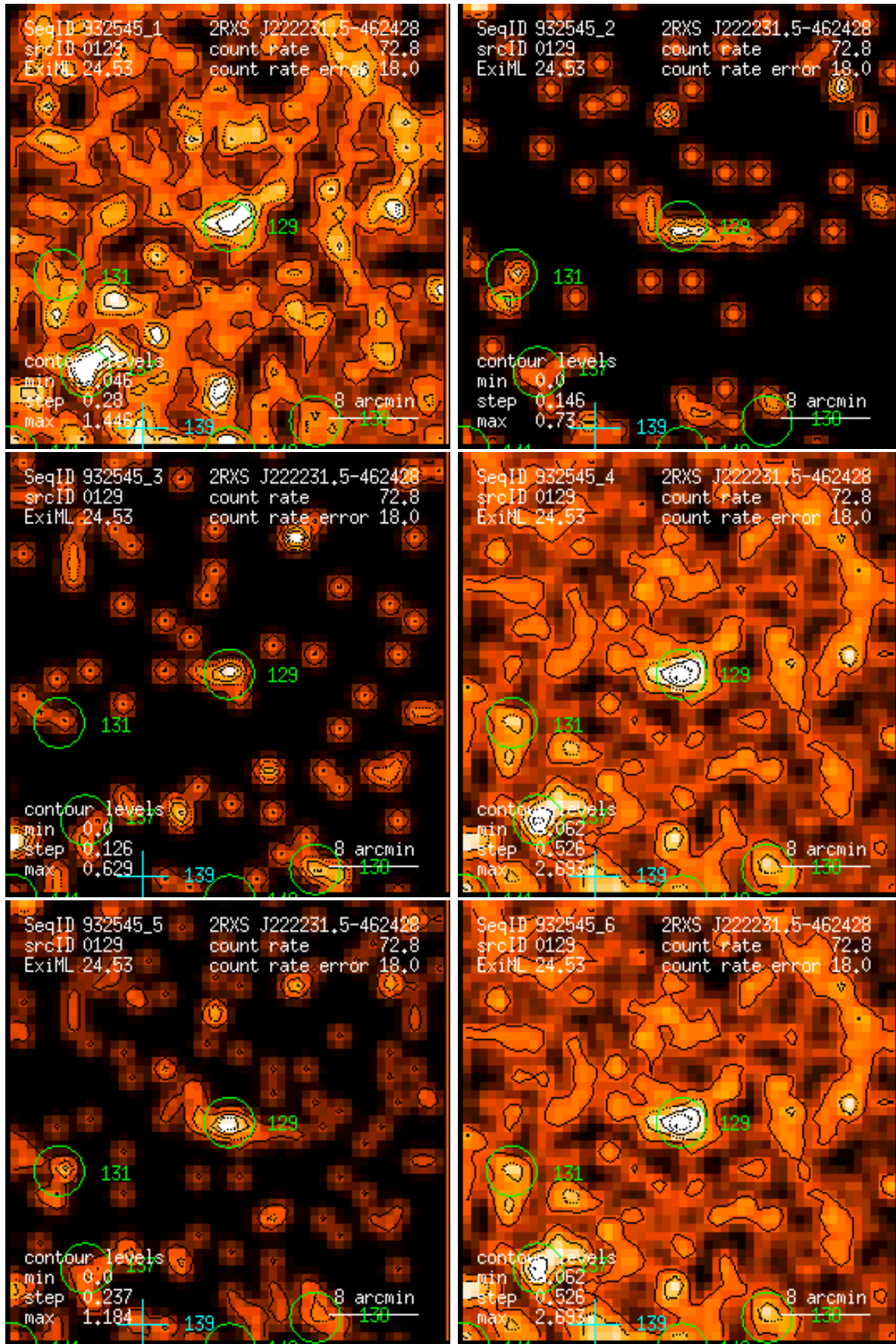
Figure 129: RASS 932545: detection 0129: band rate images, Gaussian filter: (1) PSPC channels 11 – 41, (2) 52 – 90, (3) 91 – 201, (4) 11 – 235, (5) 52 – 201, (6) 11 – 201. Broad band rates in counts/ks. Band rate contour levels in counts/ks/arcmin 2 .
