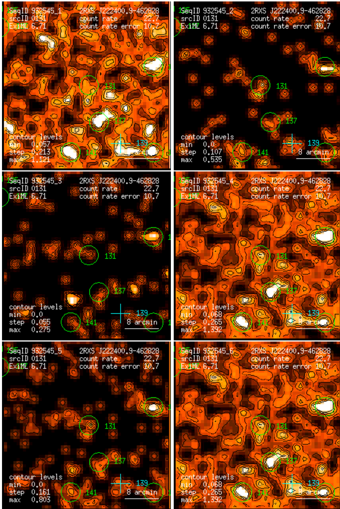
Figure 131: RASS 932545: detection 0131: band rate images, Gaussian filter: (1) PSPC channels 11 – 41, (2) 52 – 90, (3) 91 – 201, (4) 11 – 235, (5) 52 – 201, (6) 11 – 201. Broad band rates in counts/ks. Band rate contour levels in counts/ks/arcmin 2 .
