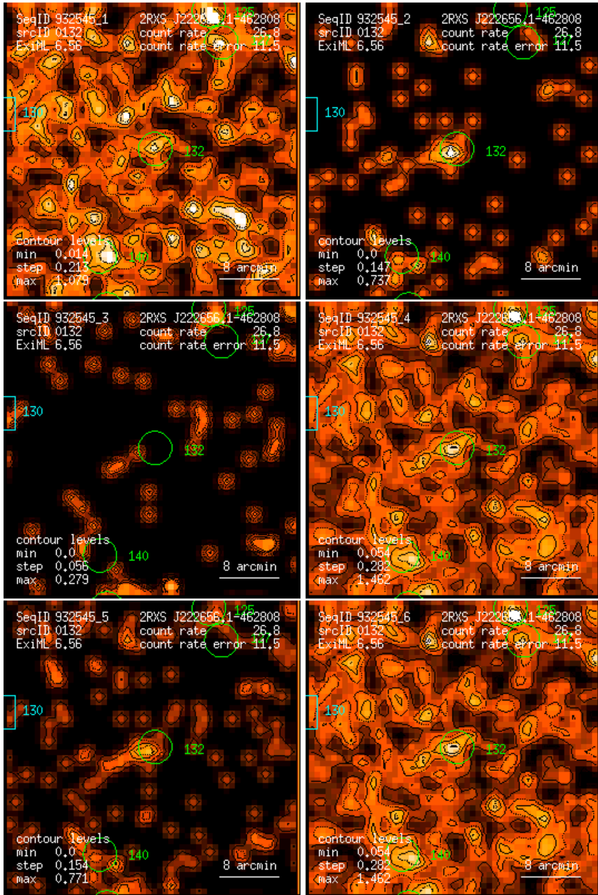
Figure 132: RASS 932545: detection 0132: band rate images, Gaussian filter: (1) PSPC channels 11 – 41, (2) 52 – 90, (3) 91 – 201, (4) 11 – 235, (5) 52 – 201, (6) 11 – 201. Broad band rates in counts/ks. Band rate contour levels in counts/ks/arcmin 2 .
