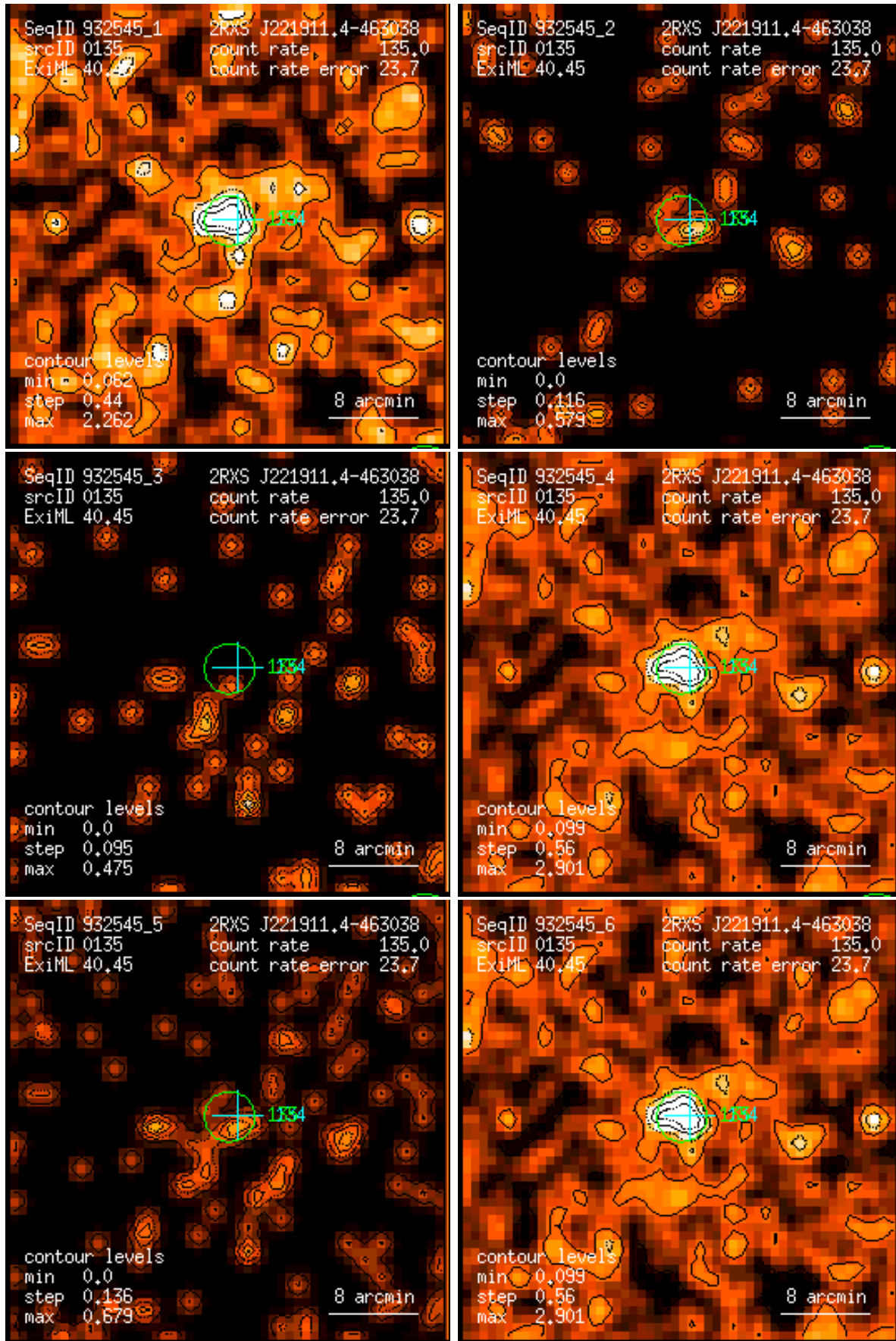
Figure 135: RASS 932545: detection 0135: band rate images, Gaussian filter: (1) PSPC channels 11 – 41, (2) 52 – 90, (3) 91 – 201, (4) 11 – 235, (5) 52 – 201, (6) 11 – 201. Broad band rates in counts/ks. Band rate contour levels in counts/ks/arcmin 2 .
