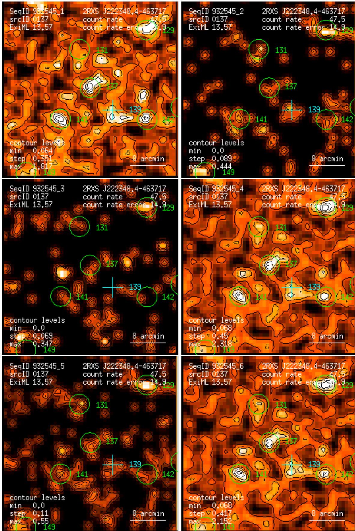
Figure 137: RASS 932545: detection 0137: band rate images, Gaussian filter: (1) PSPC channels 11 – 41, (2) 52 – 90, (3) 91 – 201, (4) 11 – 235, (5) 52 – 201, (6) 11 – 201. Broad band rates in counts/ks. Band rate contour levels in counts/ks/arcmin 2 .
