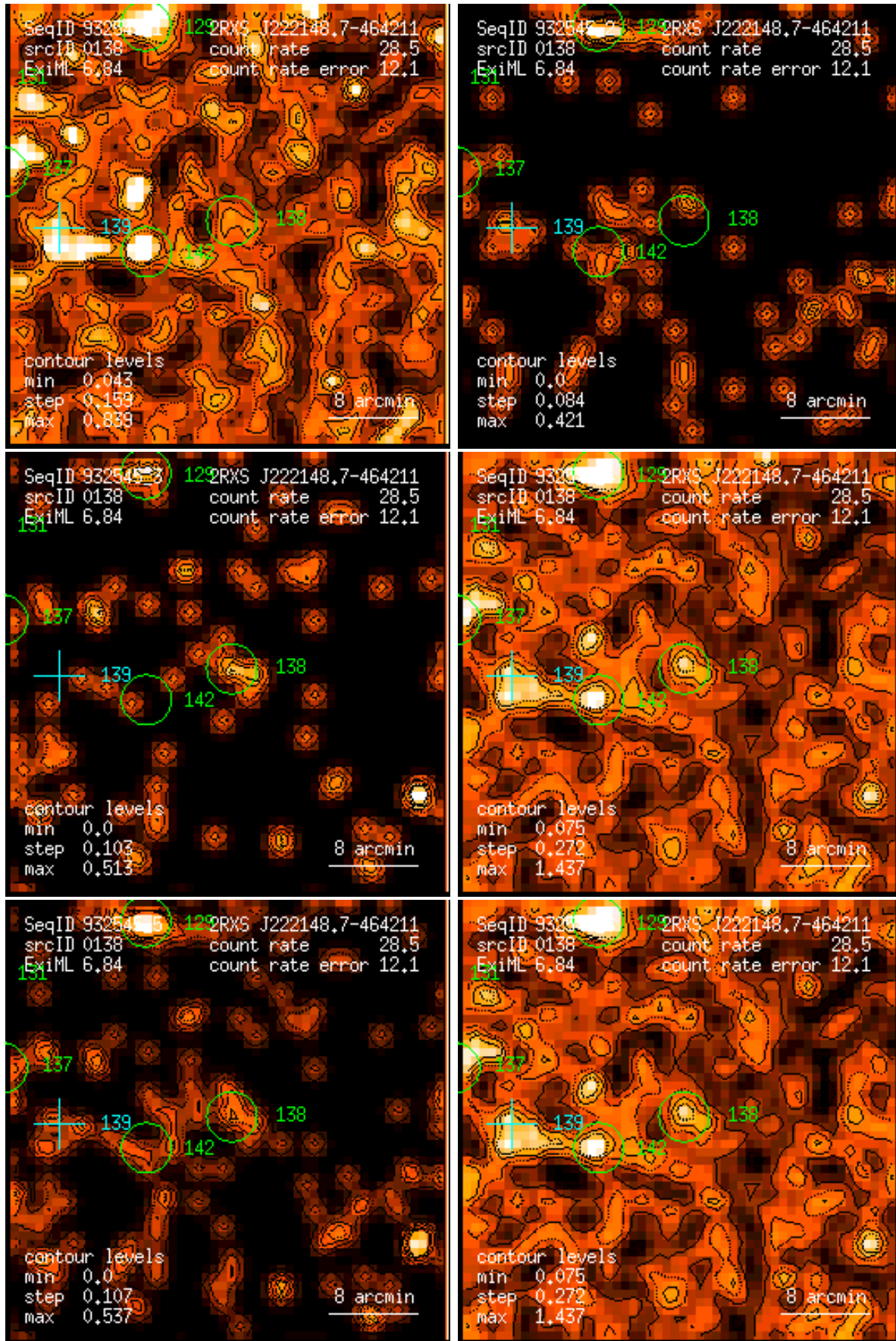
Figure 138: RASS 932545: detection 0138: band rate images, Gaussian filter: (1) PSPC channels 11 – 41, (2) 52 – 90, (3) 91 – 201, (4) 11 – 235, (5) 52 – 201, (6) 11 – 201. Broad band rates in counts/ks. Band rate contour levels in counts/ks/arcmin 2 .
