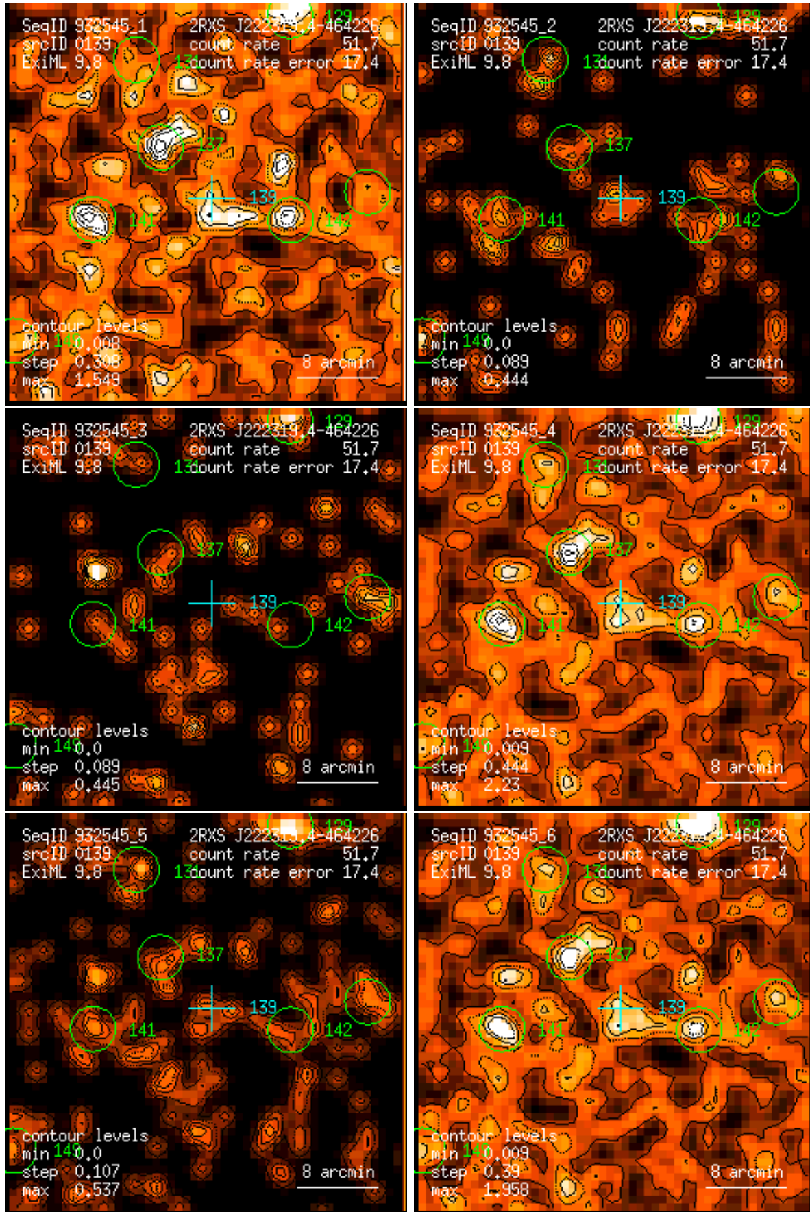
Figure 139: RASS 932545: detection 0139: band rate images, Gaussian filter: (1) PSPC channels 11 – 41, (2) 52 – 90, (3) 91 – 201, (4) 11 – 235, (5) 52 – 201, (6) 11 – 201. Broad band rates in counts/ks. Band rate contour levels in counts/ks/arcmin 2 .
