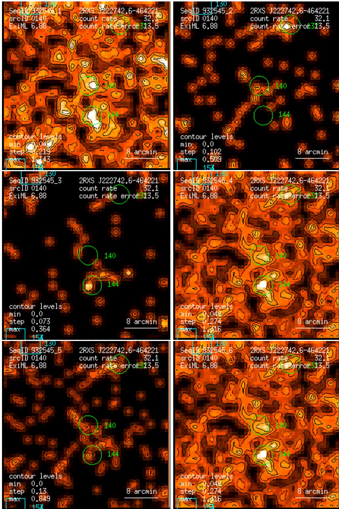
Figure 140: RASS 932545: detection 0140: band rate images, Gaussian filter: (1) PSPC channels 11 – 41, (2) 52 – 90, (3) 91 – 201, (4) 11 – 235, (5) 52 – 201, (6) 11 – 201. Broad band rates in counts/ks. Band rate contour levels in counts/ks/arcmin 2 .
