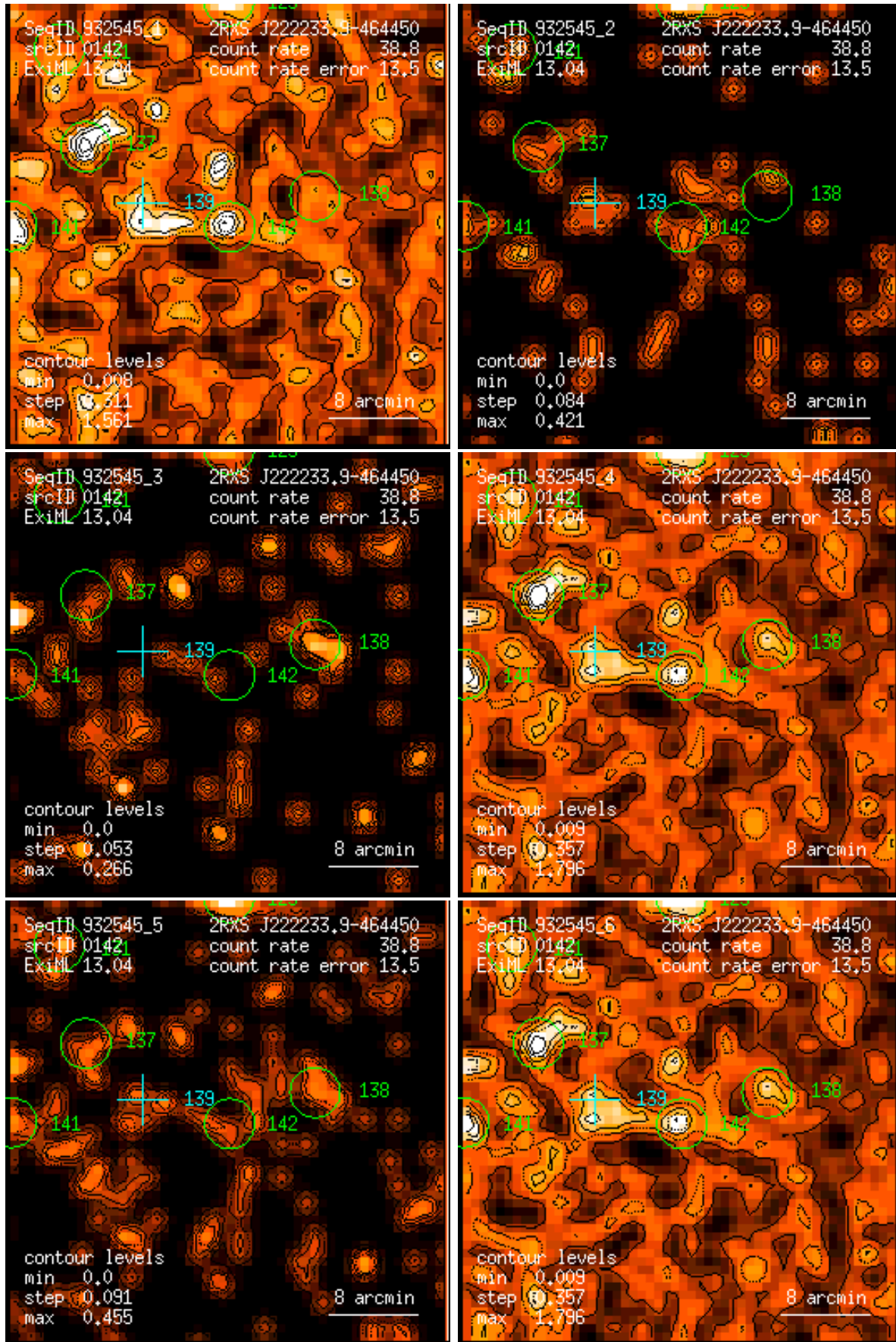
Figure 142: RASS 932545: detection 0142: band rate images, Gaussian filter: (1) PSPC channels 11 – 41, (2) 52 – 90, (3) 91 – 201, (4) 11 – 235, (5) 52 – 201, (6) 11 – 201. Broad band rates in counts/ks. Band rate contour levels in counts/ks/arcmin 2 .
