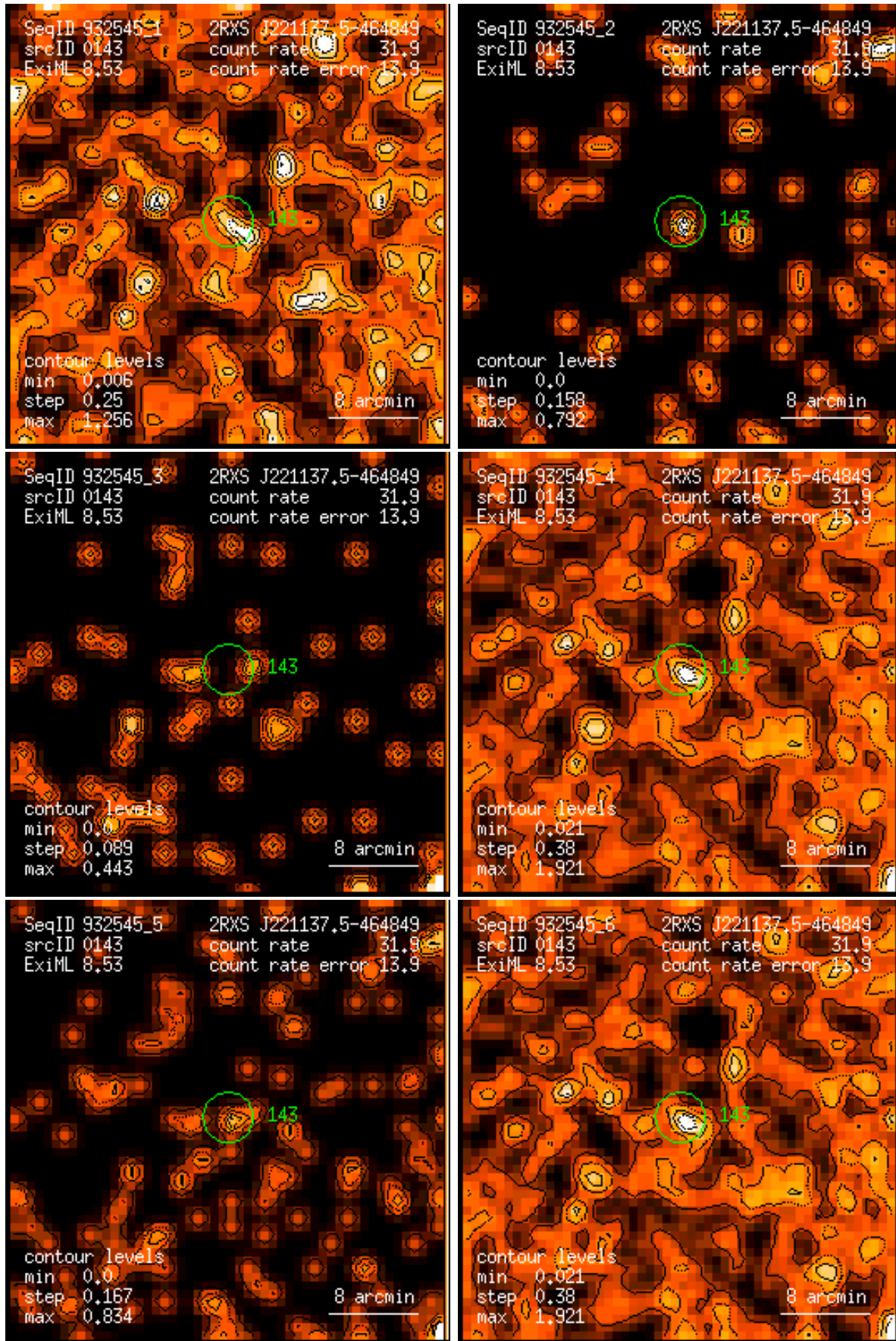
Figure 143: RASS 932545: detection 0143: band rate images, Gaussian filter: (1) PSPC channels 11 – 41, (2) 52 – 90, (3) 91 – 201, (4) 11 – 235, (5) 52 – 201, (6) 11 – 201. Broad band rates in counts/ks. Band rate contour levels in counts/ks/arcmin 2 .
