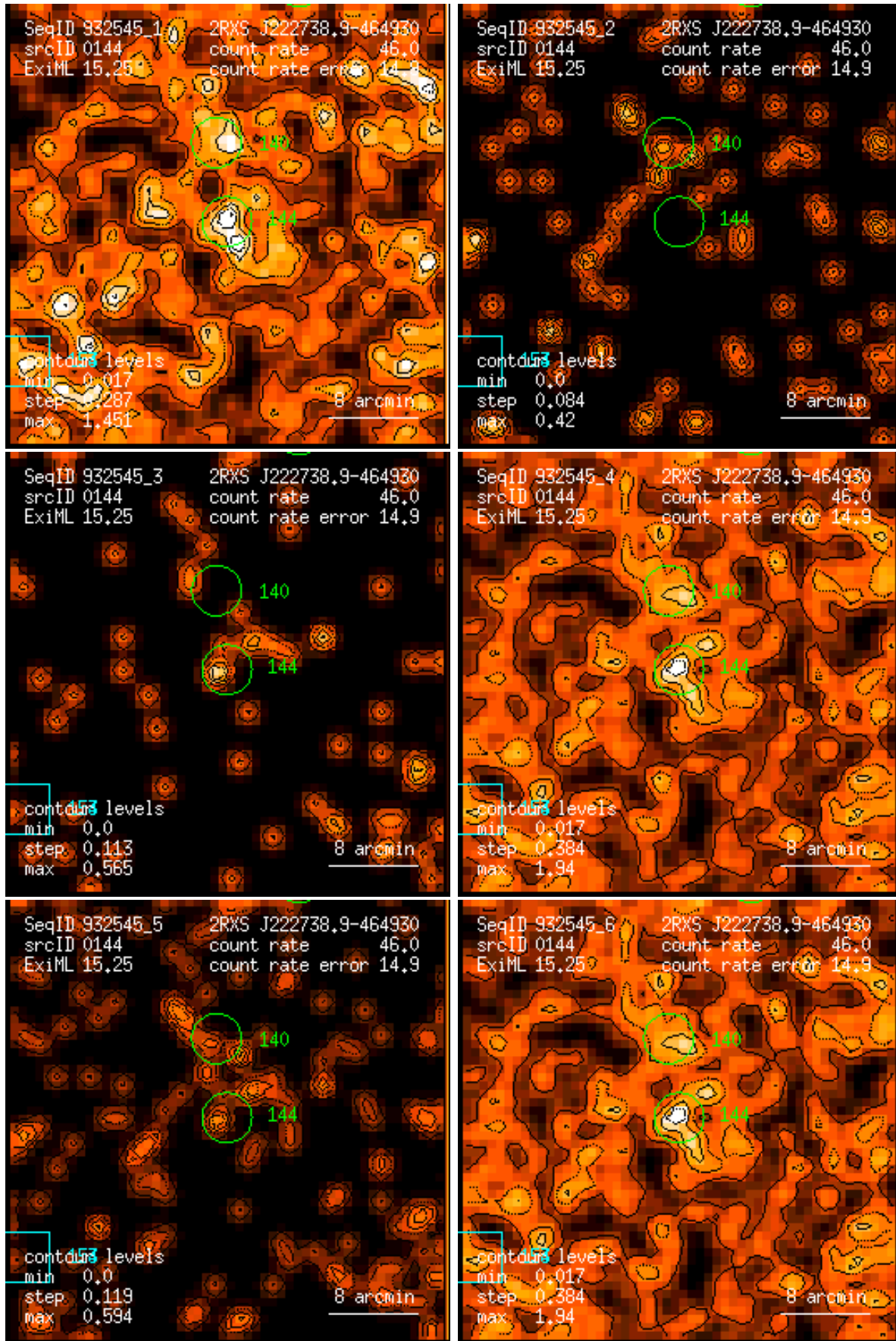
Figure 144: RASS 932545: detection 0144: band rate images, Gaussian filter: (1) PSPC channels 11 – 41, (2) 52 – 90, (3) 91 – 201, (4) 11 – 235, (5) 52 – 201, (6) 11 – 201. Broad band rates in counts/ks. Band rate contour levels in counts/ks/arcmin 2 .
