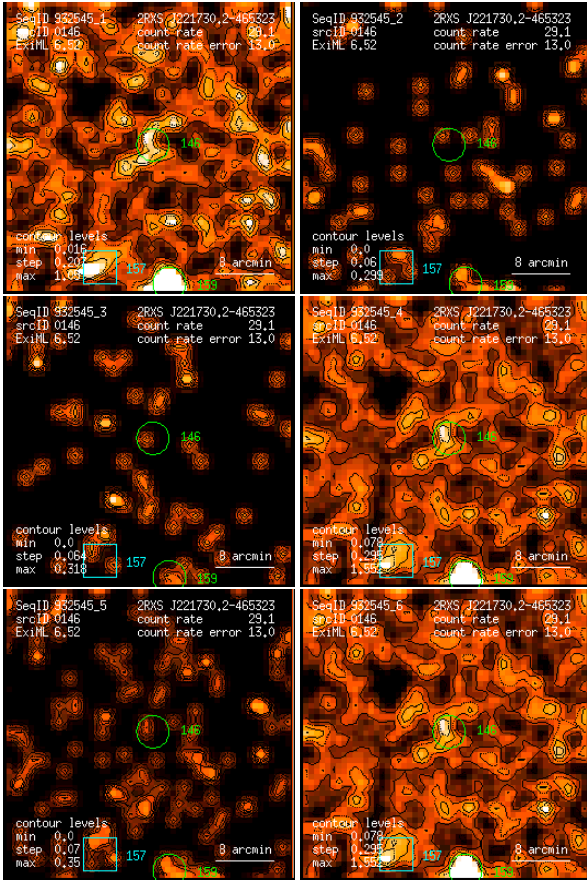
Figure 146: RASS 932545: detection 0146: band rate images, Gaussian filter: (1) PSPC channels 11 – 41, (2) 52 – 90, (3) 91 – 201, (4) 11 – 235, (5) 52 – 201, (6) 11 – 201. Broad band rates in counts/ks. Band rate contour levels in counts/ks/arcmin 2 .
