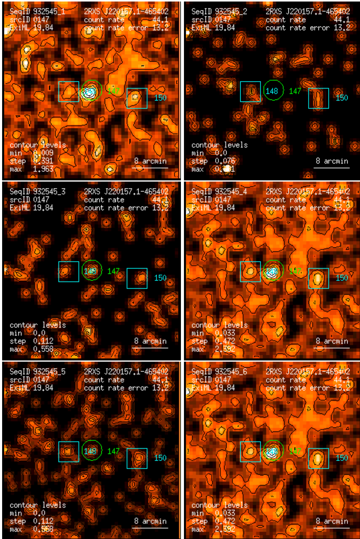
Figure 147: RASS 932545: detection 0147: band rate images, Gaussian filter: (1) PSPC channels 11 – 41, (2) 52 – 90, (3) 91 – 201, (4) 11 – 235, (5) 52 – 201, (6) 11 – 201. Broad band rates in counts/ks. Band rate contour levels in counts/ks/arcmin 2 .
