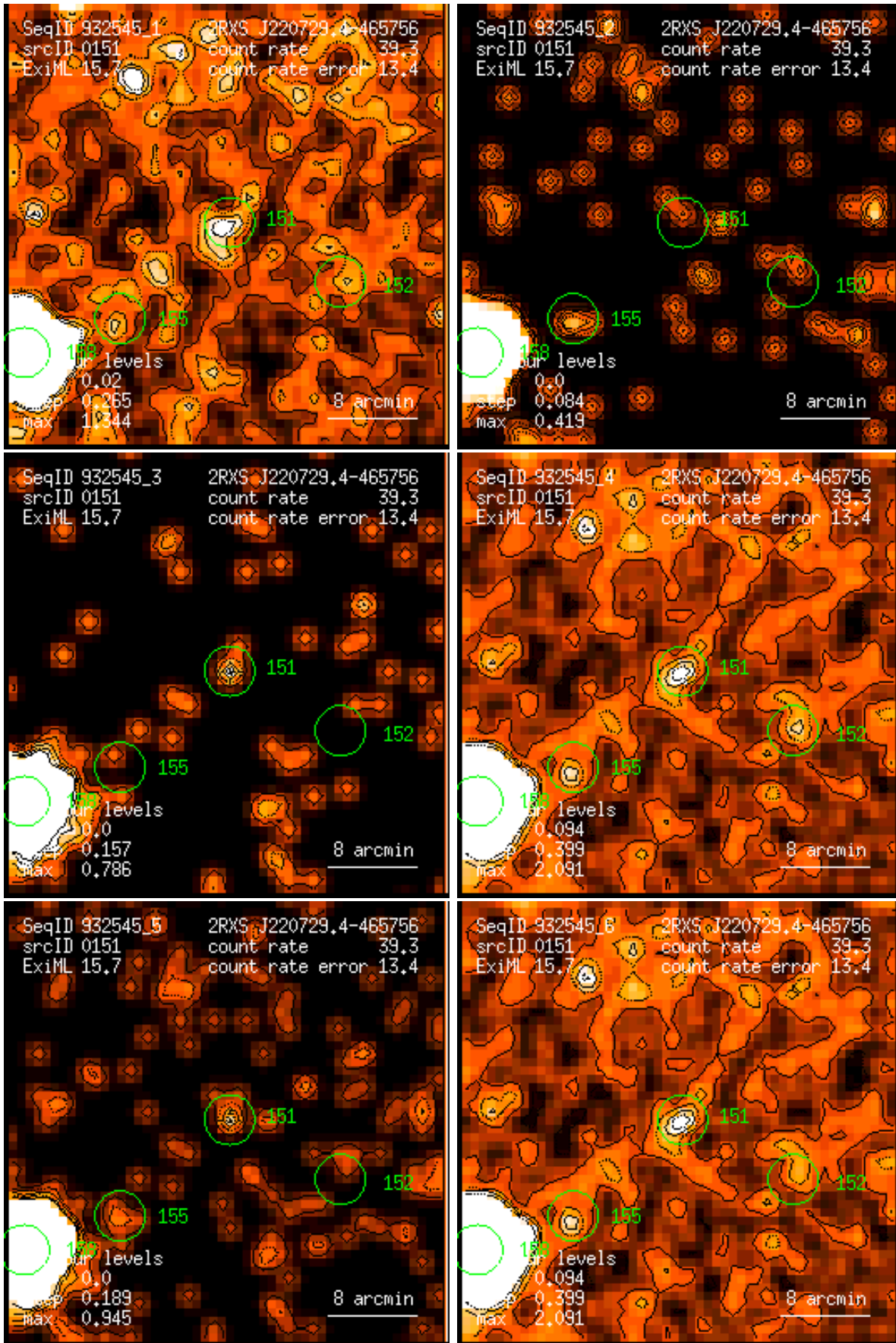
Figure 151: RASS 932545: detection 0151: band rate images, Gaussian filter: (1) PSPC channels 11 – 41, (2) 52 – 90, (3) 91 – 201, (4) 11 – 235, (5) 52 – 201, (6) 11 – 201. Broad band rates in counts/ks. Band rate contour levels in counts/ks/arcmin 2 .
