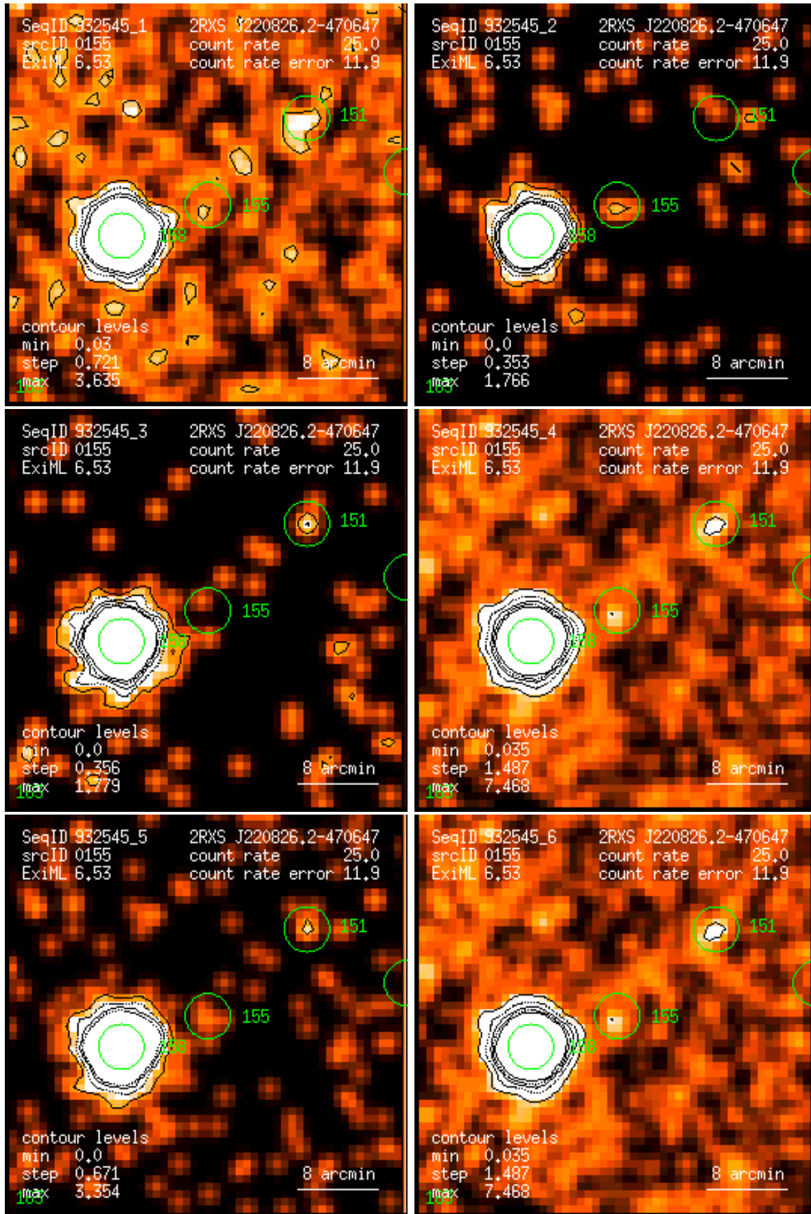
Figure 155: RASS 932545: detection 0155: band rate images, Gaussian filter: (1) PSPC channels 11 – 41, (2) 52 – 90, (3) 91 – 201, (4) 11 – 235, (5) 52 – 201, (6) 11 – 201. Broad band rates in counts/ks. Band rate contour levels in counts/ks/arcmin 2 .
