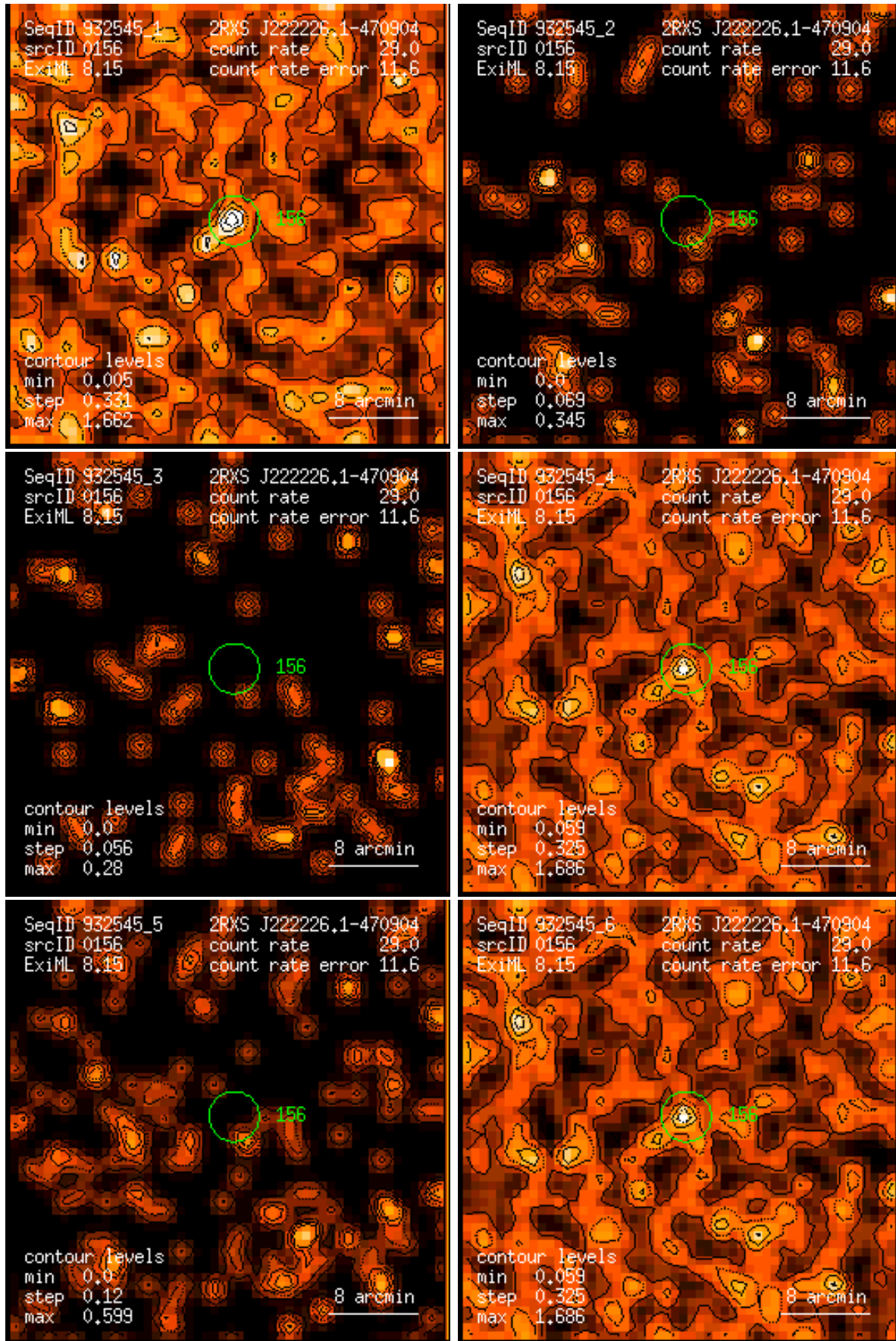
Figure 156: RASS 932545: detection 0156: band rate images, Gaussian filter: (1) PSPC channels 11 – 41, (2) 52 – 90, (3) 91 – 201, (4) 11 – 235, (5) 52 – 201, (6) 11 – 201. Broad band rates in counts/ks. Band rate contour levels in counts/ks/arcmin 2 .
