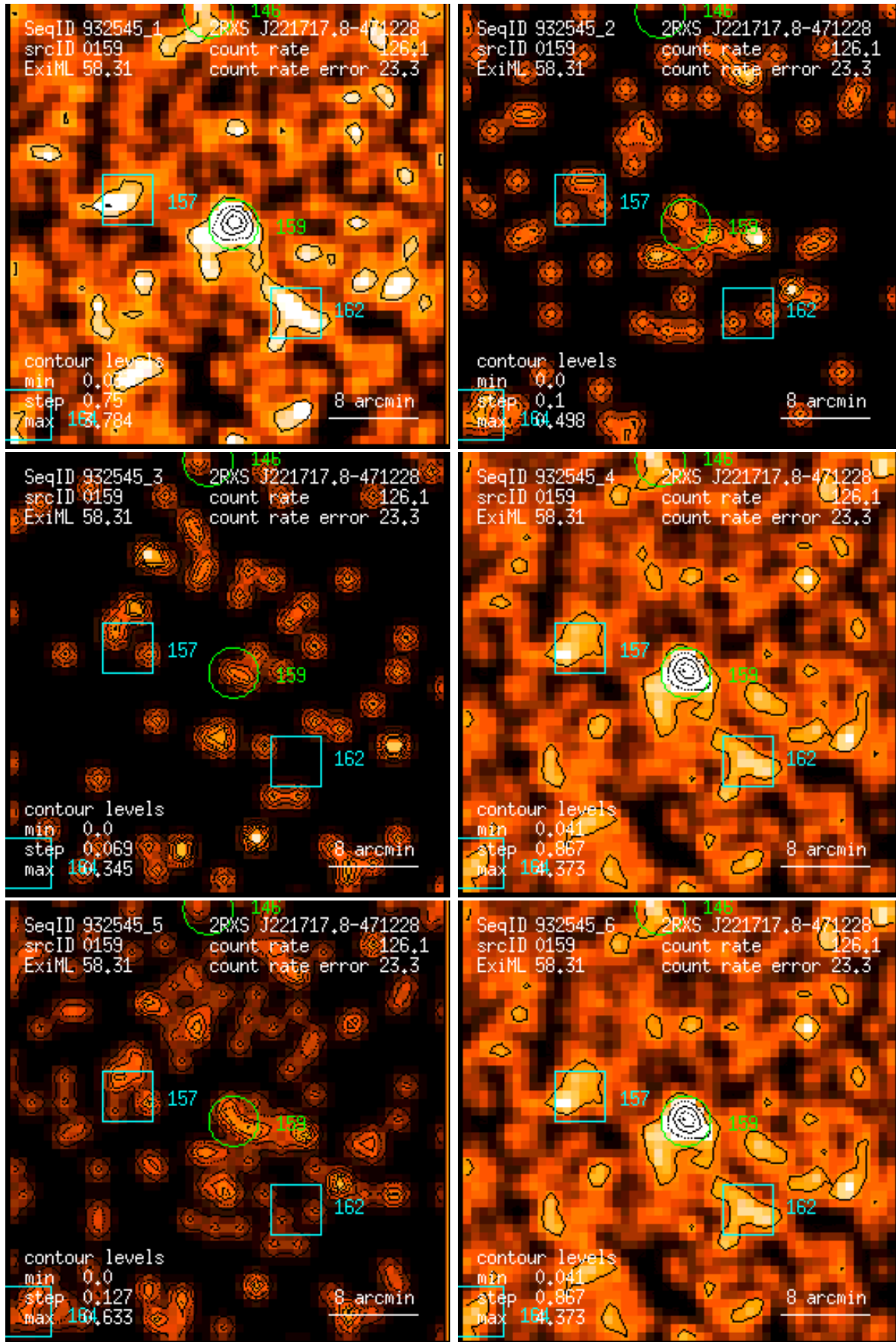
Figure 159: RASS 932545: detection 0159: band rate images, Gaussian filter: (1) PSPC channels 11 – 41, (2) 52 – 90, (3) 91 – 201, (4) 11 – 235, (5) 52 – 201, (6) 11 – 201. Broad band rates in counts/ks. Band rate contour levels in counts/ks/arcmin 2 .
