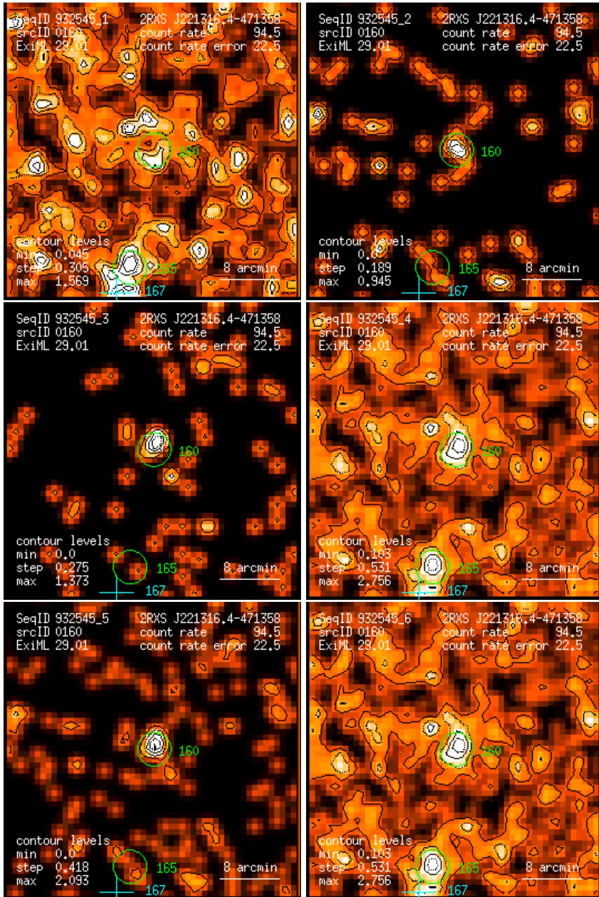
Figure 160: RASS 932545: detection 0160: band rate images, Gaussian filter: (1) PSPC channels 11 – 41, (2) 52 – 90, (3) 91 – 201, (4) 11 – 235, (5) 52 – 201, (6) 11 – 201. Broad band rates in counts/ks. Band rate contour levels in counts/ks/arcmin 2 .
