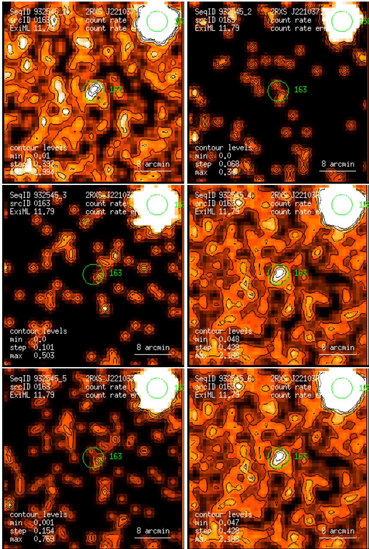
Figure 163: RASS 932545: detection 0163: band rate images, Gaussian filter: (1) PSPC channels 11 – 41, (2) 52 – 90, (3) 91 – 201, (4) 11 – 235, (5) 52 – 201, (6) 11 – 201. Broad band rates in counts/ks. Band rate contour levels in counts/ks/arcmin 2 .
