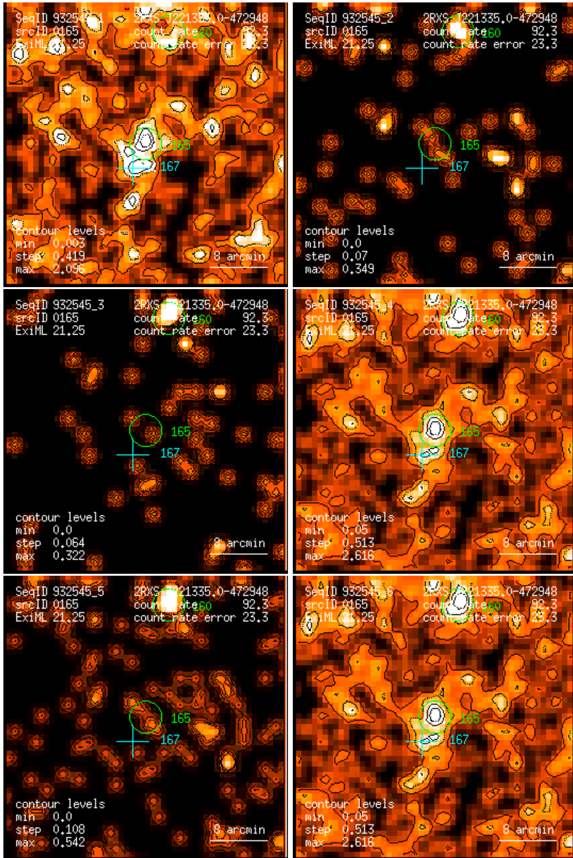
Figure 165: RASS 932545: detection 0165: band rate images, Gaussian filter: (1) PSPC channels 11 – 41, (2) 52 – 90, (3) 91 – 201, (4) 11 – 235, (5) 52 – 201, (6) 11 – 201. Broad band rates in counts/ks. Band rate contour levels in counts/ks/arcmin 2 .
