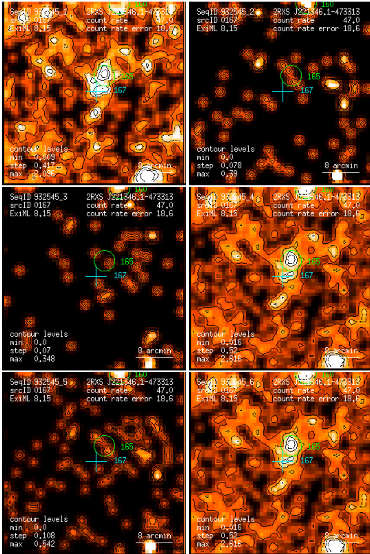
Figure 167: RASS 932545: detection 0167: band rate images, Gaussian filter: (1) PSPC channels 11 – 41, (2) 52 – 90, (3) 91 – 201, (4) 11 – 235, (5) 52 – 201, (6) 11 – 201. Broad band rates in counts/ks. Band rate contour levels in counts/ks/arcmin 2 .
