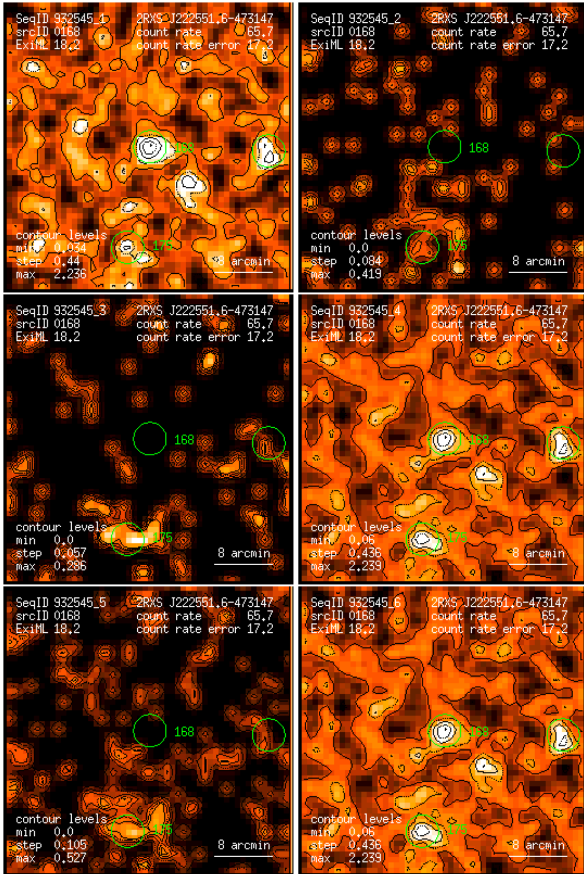
Figure 168: RASS 932545: detection 0168: band rate images, Gaussian filter: (1) PSPC channels 11 – 41, (2) 52 – 90, (3) 91 – 201, (4) 11 – 235, (5) 52 – 201, (6) 11 – 201. Broad band rates in counts/ks. Band rate contour levels in counts/ks/arcmin 2 .
