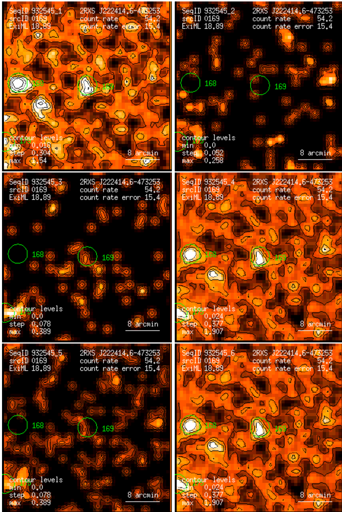
Figure 169: RASS 932545: detection 0169: band rate images, Gaussian filter: (1) PSPC channels 11 – 41, (2) 52 – 90, (3) 91 – 201, (4) 11 – 235, (5) 52 – 201, (6) 11 – 201. Broad band rates in counts/ks. Band rate contour levels in counts/ks/arcmin 2 .
